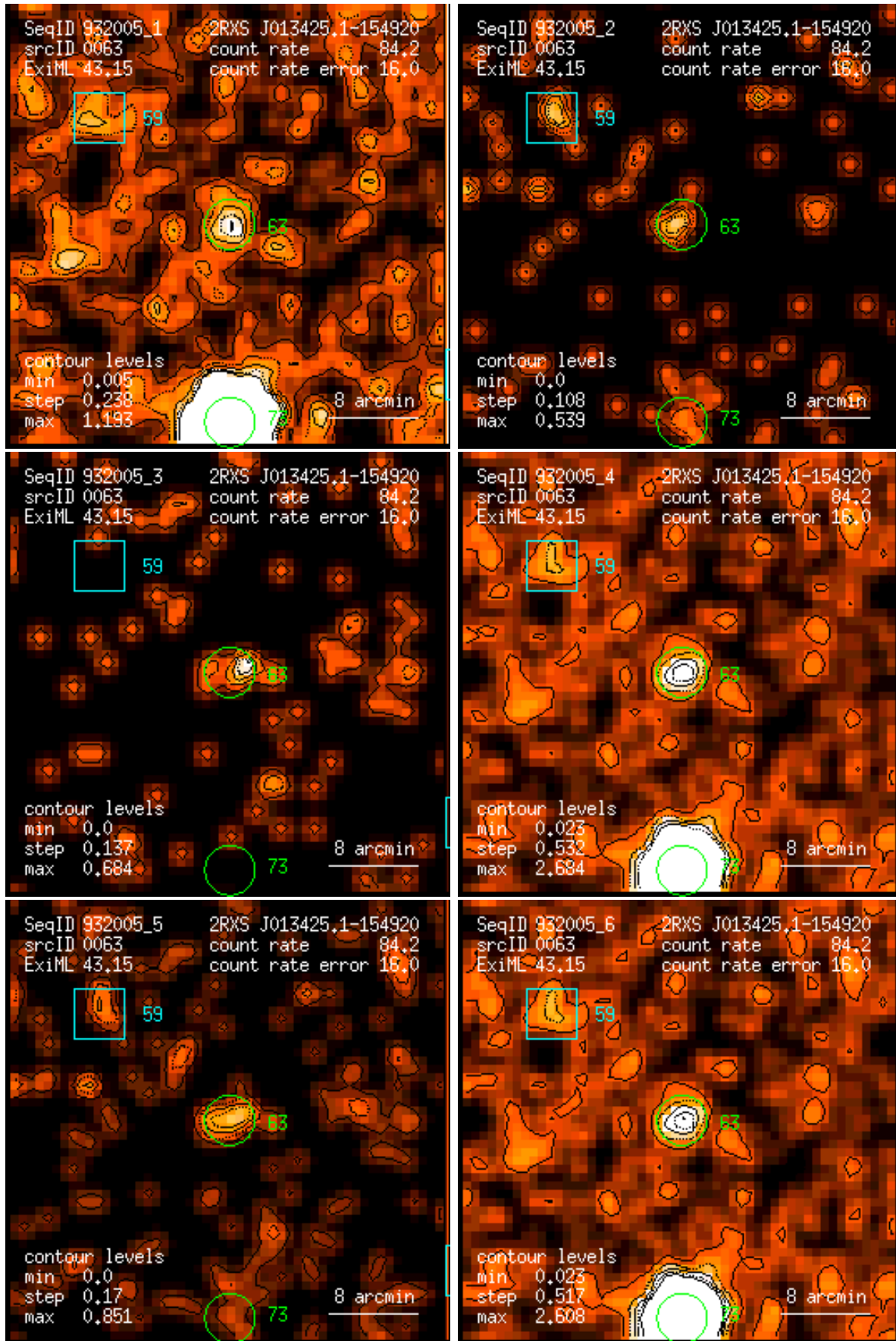
Figure 63: RASS 932005: detection 0063: band rate images, Gaussian filter: (1) PSPC channels 11 – 41, (2) 52 – 90, (3) 91 – 201, (4) 11 – 235, (5) 52 – 201, (6) 11 – 201. Broad band rates in counts/ks. Band rate contour levels in counts/ks/arcmin 2 .
