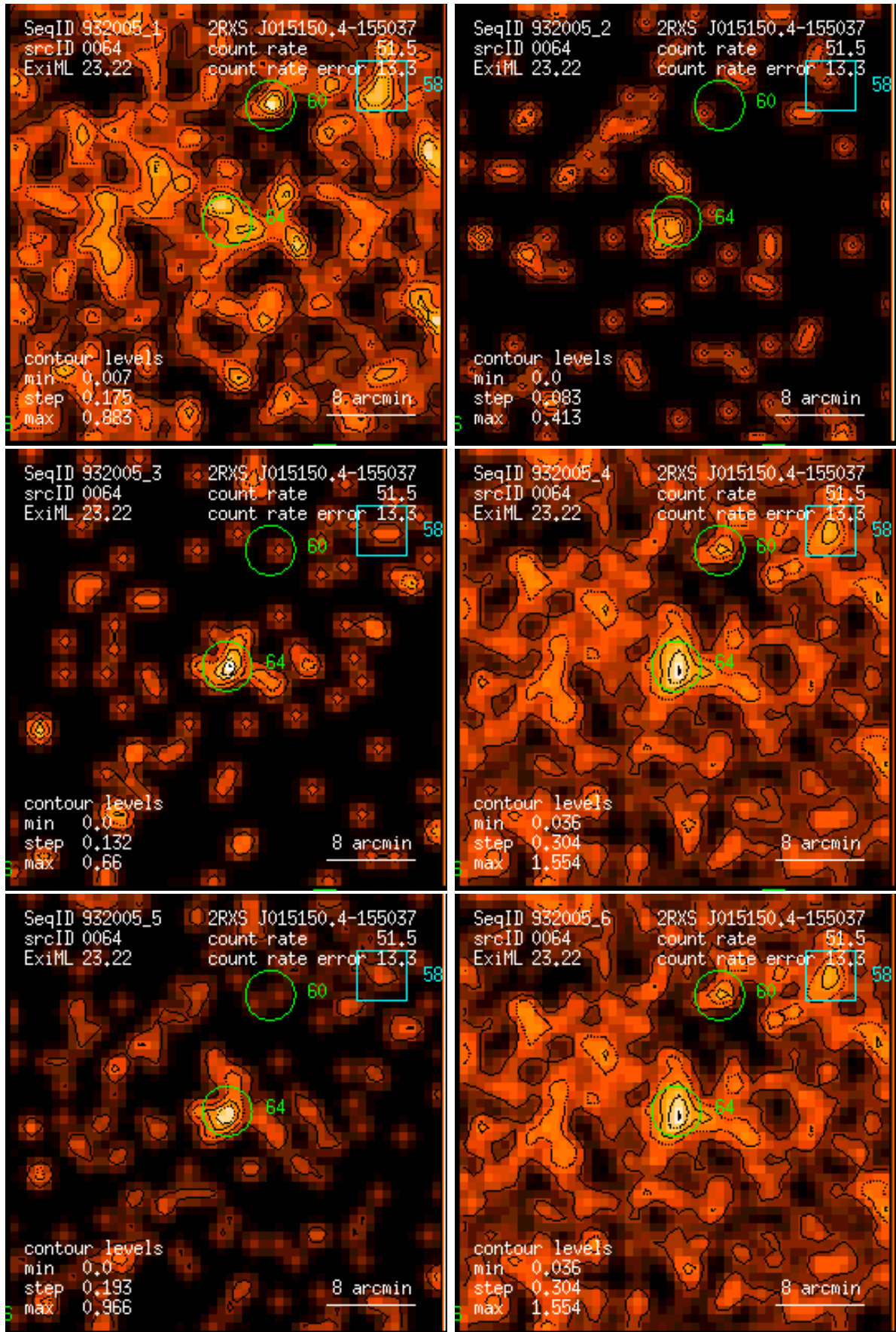
Figure 64: RASS 932005: detection 0064: band rate images, Gaussian filter: (1) PSPC channels 11 – 41, (2) 52 – 90, (3) 91 – 201, (4) 11 – 235, (5) 52 – 201, (6) 11 – 201. Broad band rates in counts/ks. Band rate contour levels in counts/ks/arcmin 2 .
