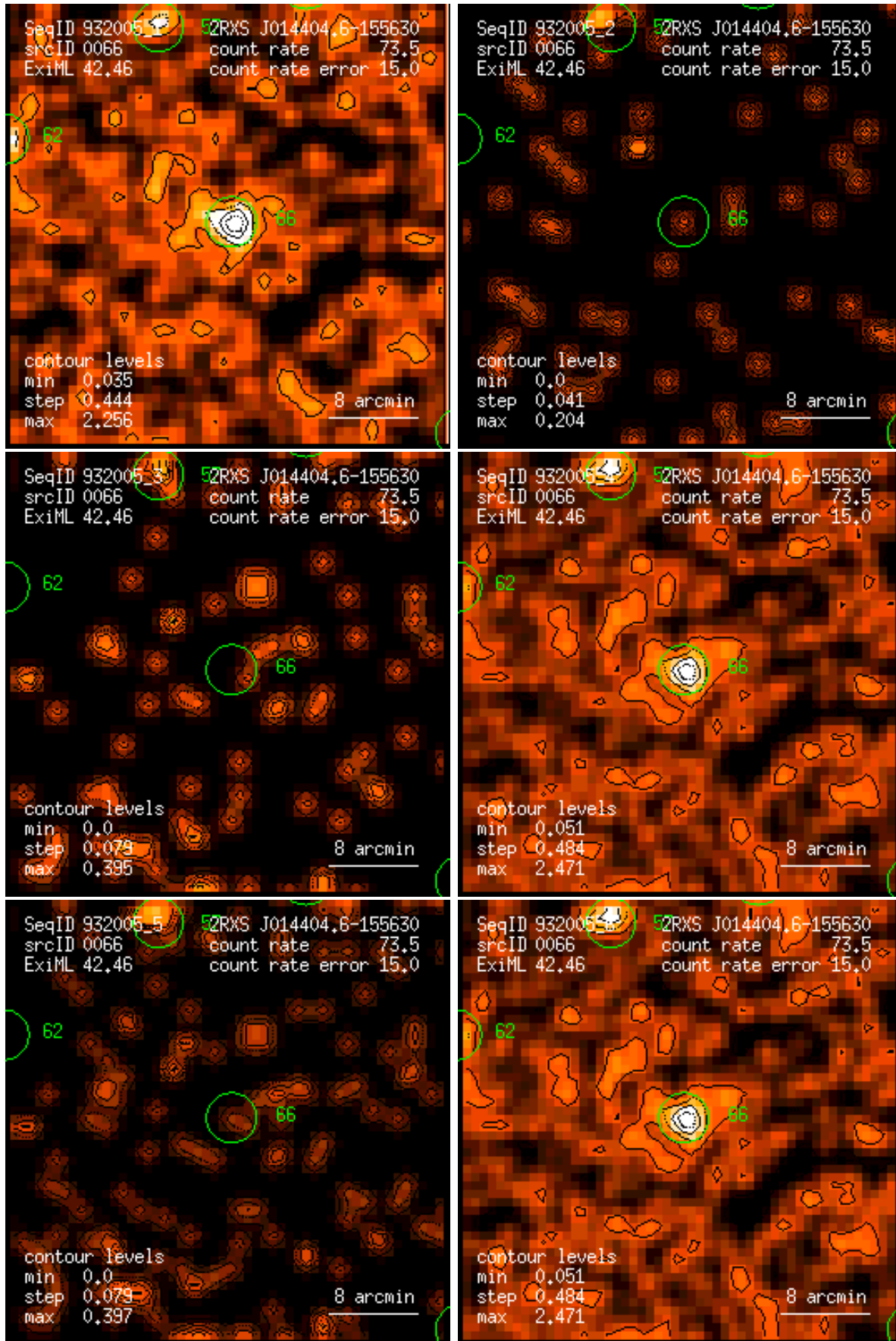
Figure 66: RASS 932005: detection 0066: band rate images, Gaussian filter: (1) PSPC channels 11 – 41, (2) 52 – 90, (3) 91 – 201, (4) 11 – 235, (5) 52 – 201, (6) 11 – 201. Broad band rates in counts/ks. Band rate contour levels in counts/ks/arcmin 2 .
