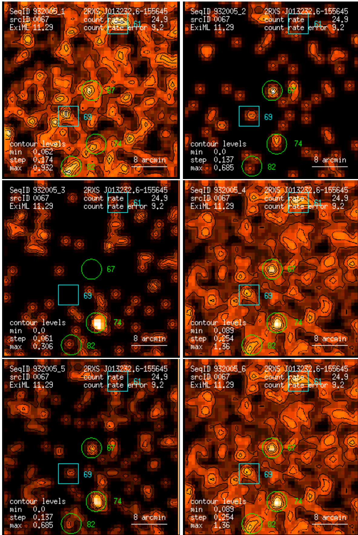
Figure 67: RASS 932005: detection 0067: band rate images, Gaussian filter: (1) PSPC channels 11 – 41, (2) 52 – 90, (3) 91 – 201, (4) 11 – 235, (5) 52 – 201, (6) 11 – 201. Broad band rates in counts/ks. Band rate contour levels in counts/ks/arcmin 2 .
