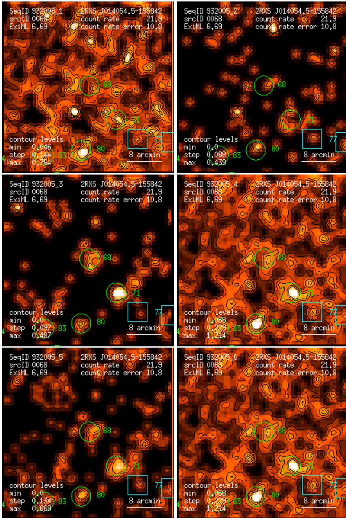
Figure 68: RASS 932005: detection 0068: band rate images, Gaussian filter: (1) PSPC channels 11 – 41, (2) 52 – 90, (3) 91 – 201, (4) 11 – 235, (5) 52 – 201, (6) 11 – 201. Broad band rates in counts/ks. Band rate contour levels in counts/ks/arcmin 2 .
