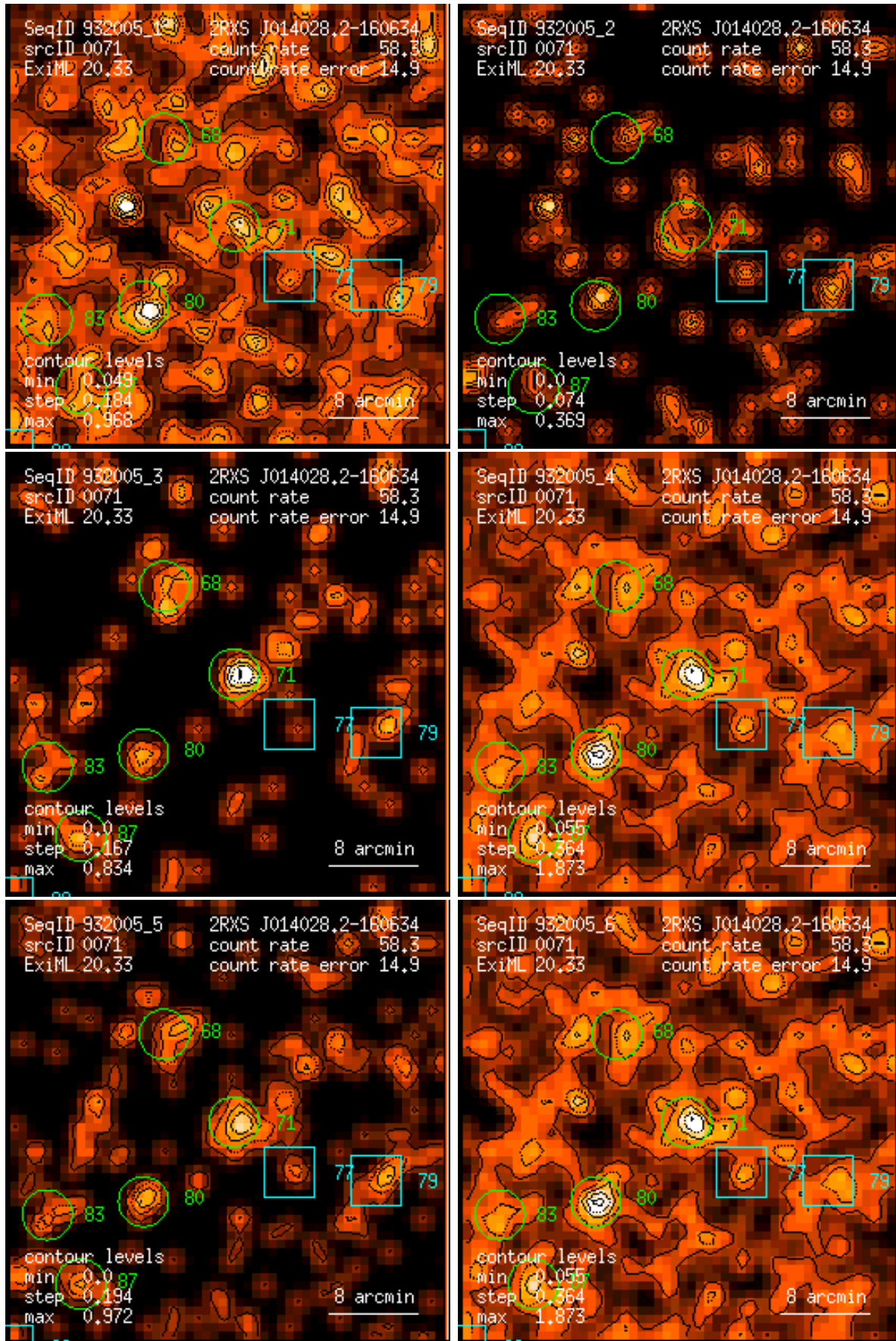
Figure 71: RASS 932005: detection 0071: band rate images, Gaussian filter: (1) PSPC channels 11 – 41, (2) 52 – 90, (3) 91 – 201, (4) 11 – 235, (5) 52 – 201, (6) 11 – 201. Broad band rates in counts/ks. Band rate contour levels in counts/ks/arcmin 2 .
