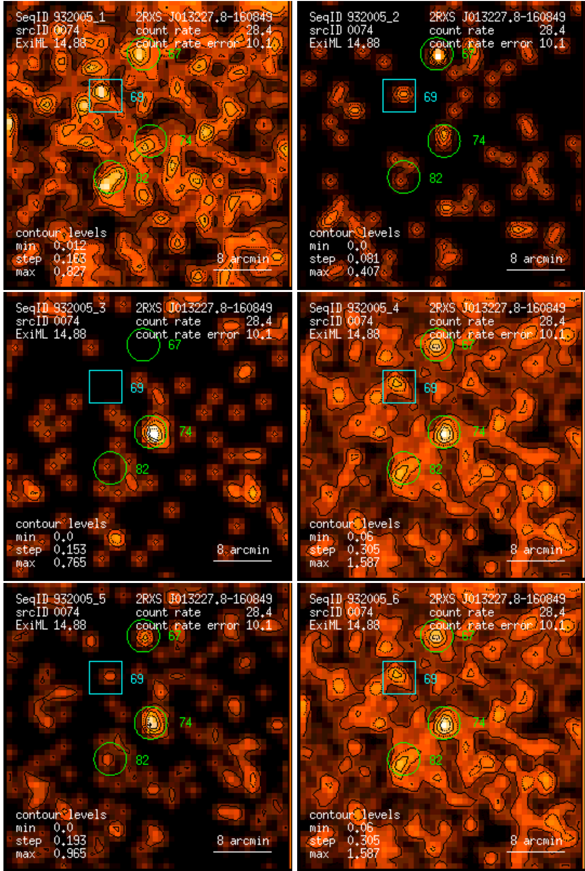
Figure 74: RASS 932005: detection 0074: band rate images, Gaussian filter: (1) PSPC channels 11 – 41, (2) 52 – 90, (3) 91 – 201, (4) 11 – 235, (5) 52 – 201, (6) 11 – 201. Broad band rates in counts/ks. Band rate contour levels in counts/ks/arcmin 2 .
