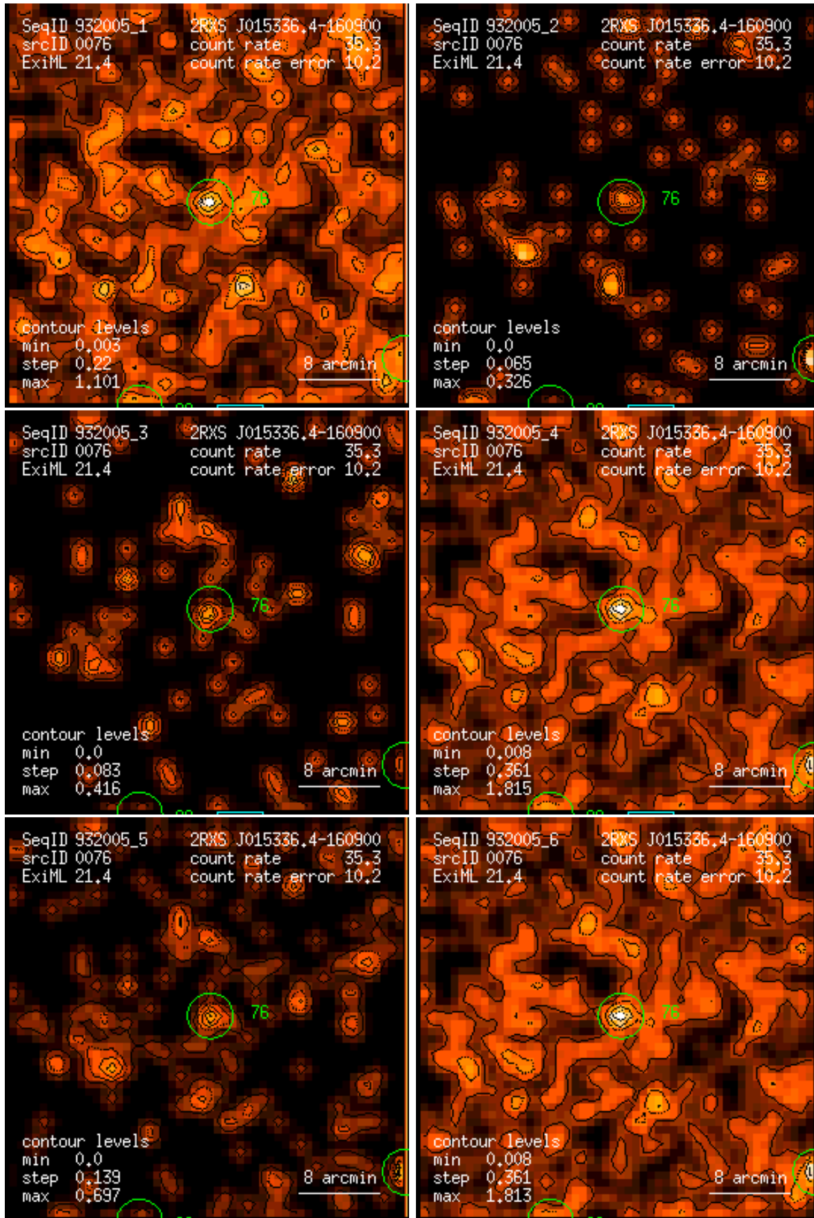
Figure 76: RASS 932005: detection 0076: band rate images, Gaussian filter: (1) PSPC channels 11 – 41, (2) 52 – 90, (3) 91 – 201, (4) 11 – 235, (5) 52 – 201, (6) 11 – 201. Broad band rates in counts/ks. Band rate contour levels in counts/ks/arcmin 2 .
