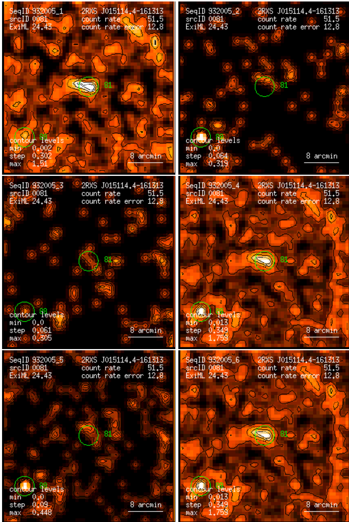
Figure 81: RASS 932005: detection 0081: band rate images, Gaussian filter: (1) PSPC channels 11 – 41, (2) 52 – 90, (3) 91 – 201, (4) 11 – 235, (5) 52 – 201, (6) 11 – 201. Broad band rates in counts/ks. Band rate contour levels in counts/ks/arcmin 2 .
