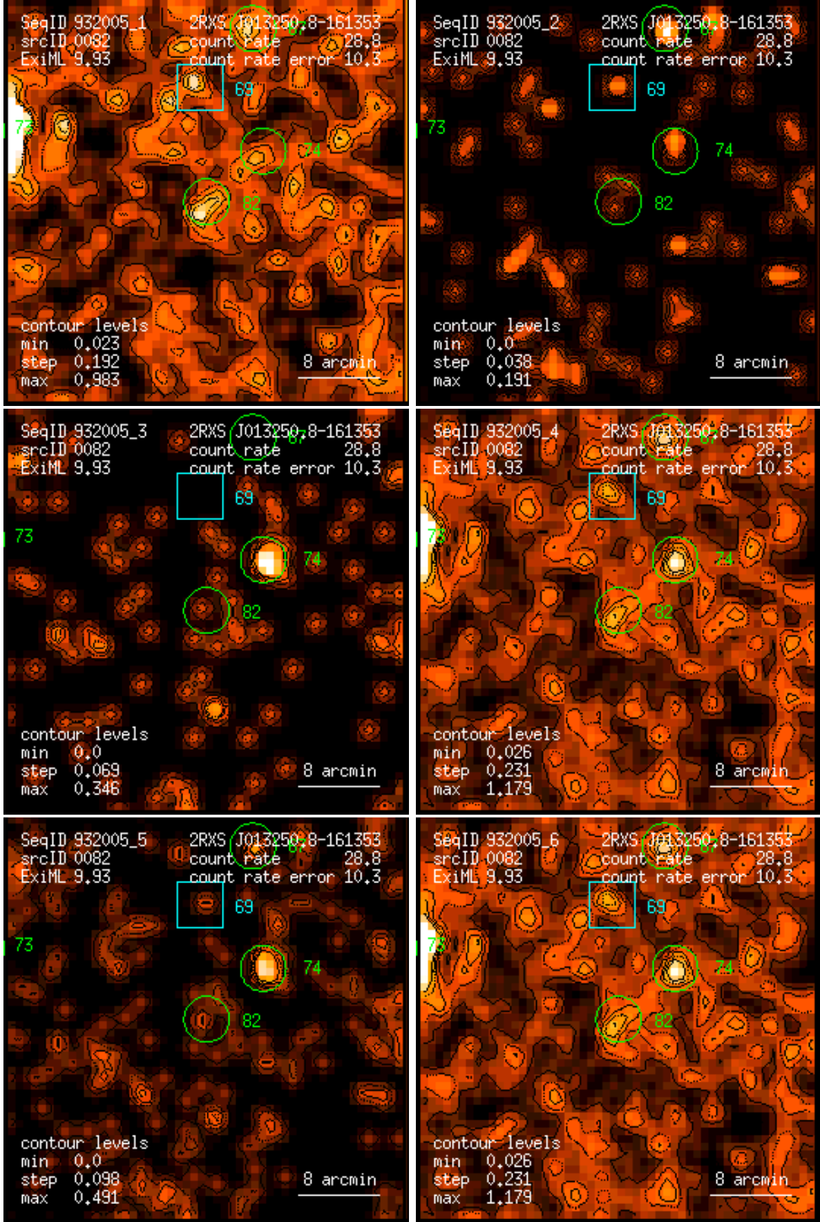
Figure 82: RASS 932005: detection 0082: band rate images, Gaussian filter: (1) PSPC channels 11 – 41, (2) 52 – 90, (3) 91 – 201, (4) 11 – 235, (5) 52 – 201, (6) 11 – 201. Broad band rates in counts/ks. Band rate contour levels in counts/ks/arcmin 2 .
