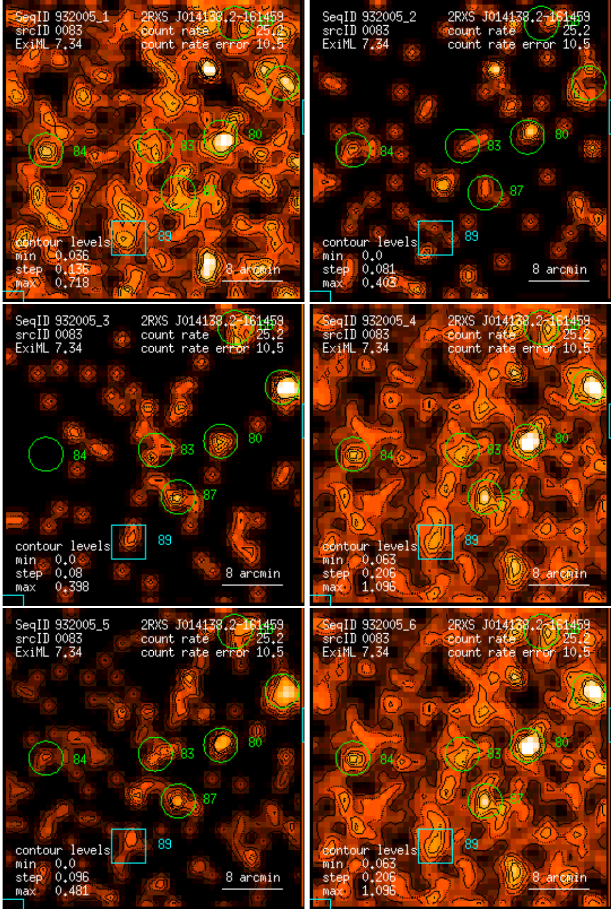
Figure 83: RASS 932005: detection 0083: band rate images, Gaussian filter: (1) PSPC channels 11 – 41, (2) 52 – 90, (3) 91 – 201, (4) 11 – 235, (5) 52 – 201, (6) 11 – 201. Broad band rates in counts/ks. Band rate contour levels in counts/ks/arcmin 2 .
