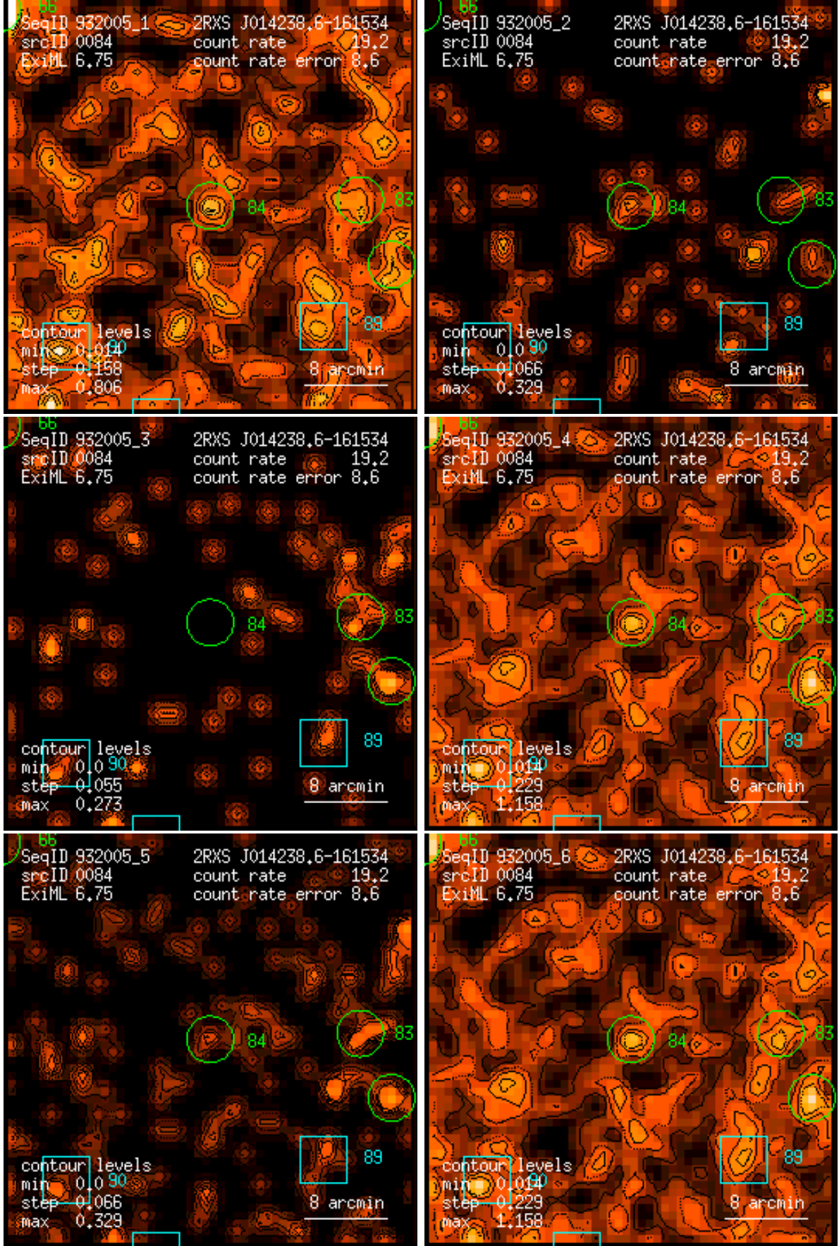
Figure 84: RASS 932005: detection 0084: band rate images, Gaussian filter: (1) PSPC channels 11 – 41, (2) 52 – 90, (3) 91 – 201, (4) 11 – 235, (5) 52 – 201, (6) 11 – 201. Broad band rates in counts/ks. Band rate contour levels in counts/ks/arcmin 2 .
