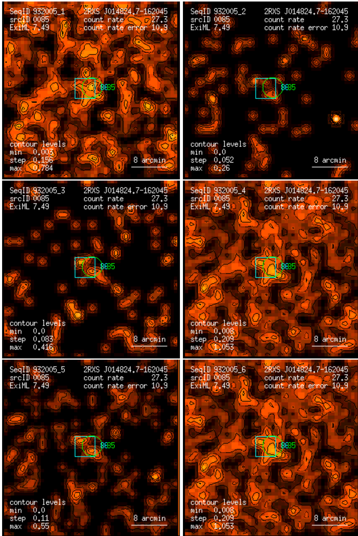
Figure 85: RASS 932005: detection 0085: band rate images, Gaussian filter: (1) PSPC channels 11 – 41, (2) 52 – 90, (3) 91 – 201, (4) 11 – 235, (5) 52 – 201, (6) 11 – 201. Broad band rates in counts/ks. Band rate contour levels in counts/ks/arcmin 2 .
