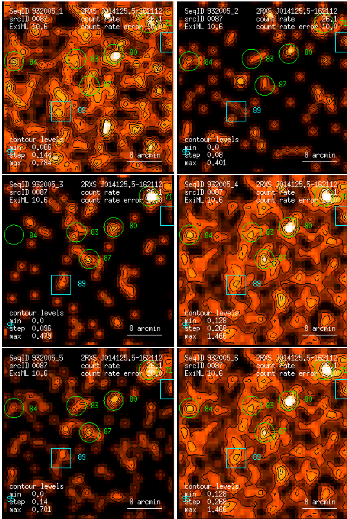
Figure 87: RASS 932005: detection 0087: band rate images, Gaussian filter: (1) PSPC channels 11 – 41, (2) 52 – 90, (3) 91 – 201, (4) 11 – 235, (5) 52 – 201, (6) 11 – 201. Broad band rates in counts/ks. Band rate contour levels in counts/ks/arcmin 2 .
