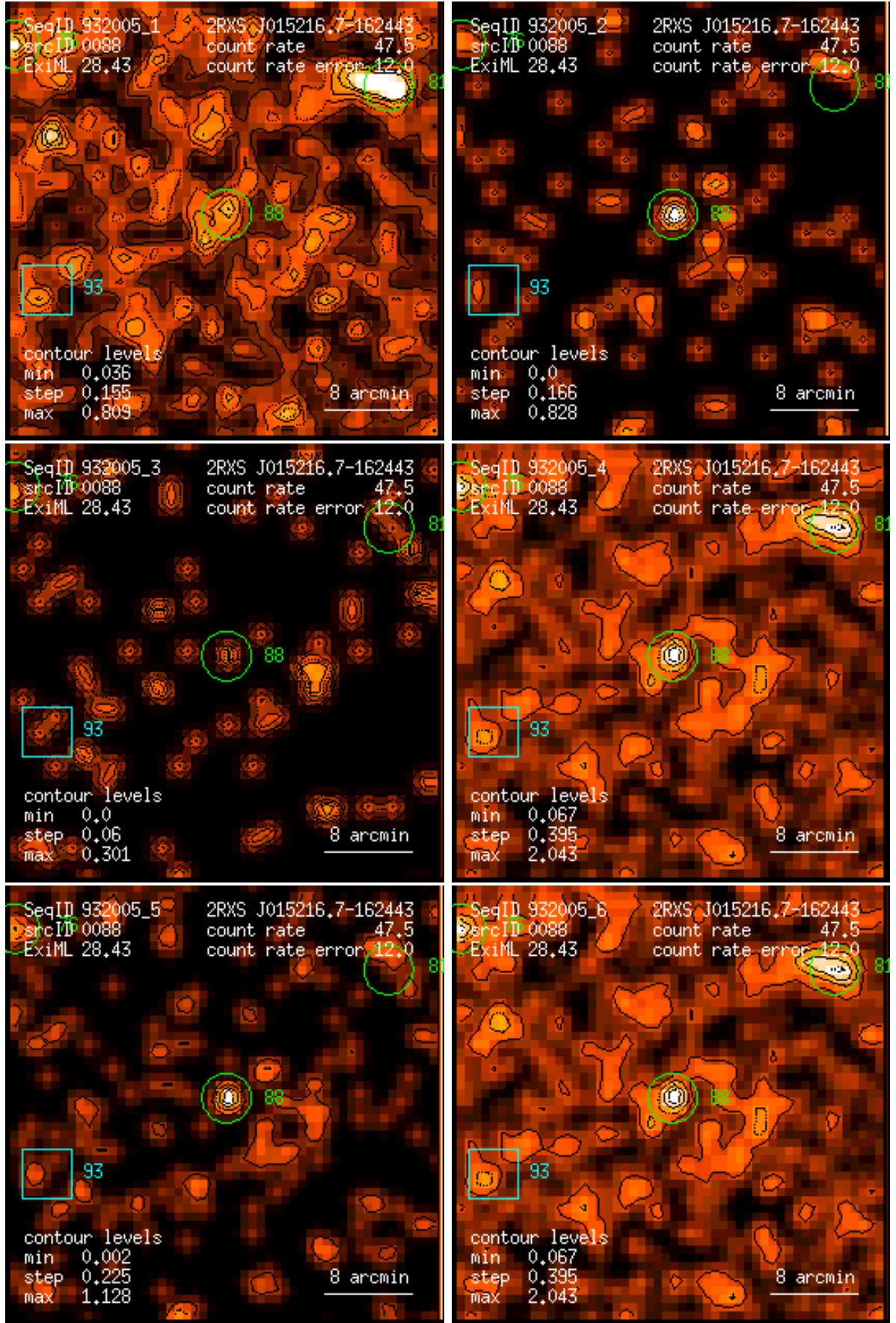
Figure 88: RASS 932005: detection 0088: band rate images, Gaussian filter: (1) PSPC channels 11 – 41, (2) 52 – 90, (3) 91 – 201, (4) 11 – 235, (5) 52 – 201, (6) 11 – 201. Broad band rates in counts/ks. Band rate contour levels in counts/ks/arcmin 2 .
