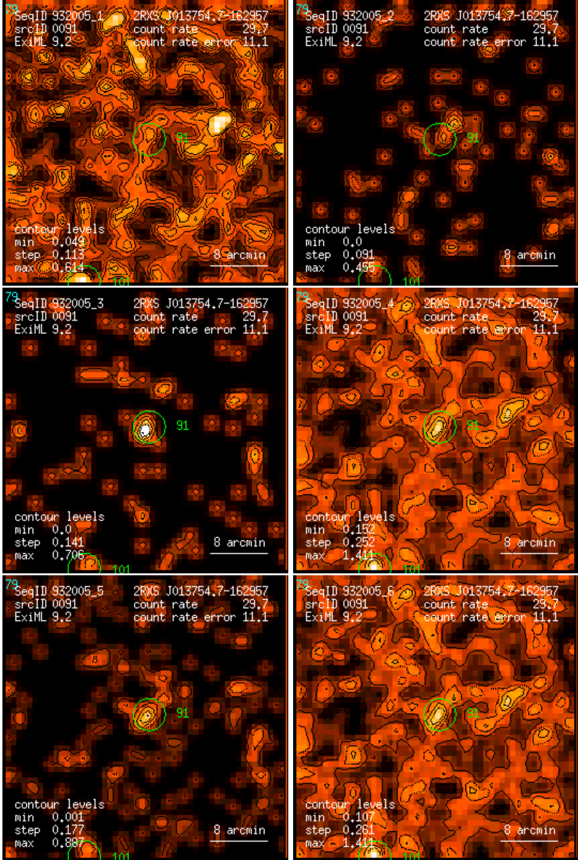
Figure 91: RASS 932005: detection 0091: band rate images, Gaussian filter: (1) PSPC channels 11 – 41, (2) 52 – 90, (3) 91 – 201, (4) 11 – 235, (5) 52 – 201, (6) 11 – 201. Broad band rates in counts/ks. Band rate contour levels in counts/ks/arcmin 2 .
