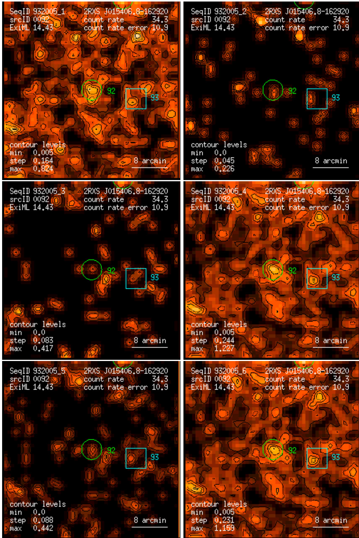
Figure 92: RASS 932005: detection 0092: band rate images, Gaussian filter: (1) PSPC channels 11 – 41, (2) 52 – 90, (3) 91 – 201, (4) 11 – 235, (5) 52 – 201, (6) 11 – 201. Broad band rates in counts/ks. Band rate contour levels in counts/ks/arcmin 2 .
