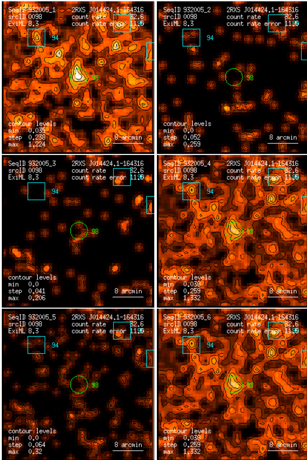
Figure 98: RASS 932005: detection 0098: band rate images, Gaussian filter: (1) PSPC channels 11 – 41, (2) 52 – 90, (3) 91 – 201, (4) 11 – 235, (5) 52 – 201, (6) 11 – 201. Broad band rates in counts/ks. Band rate contour levels in counts/ks/arcmin 2 .
