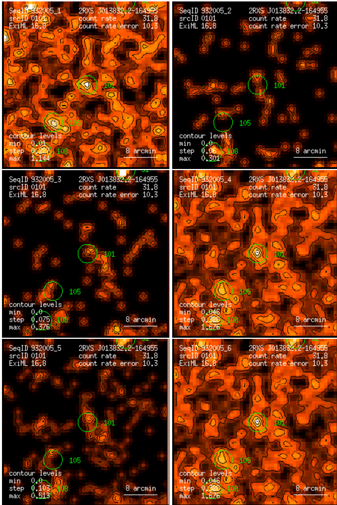
Figure 101: RASS 932005: detection 0101: band rate images, Gaussian filter: (1) PSPC channels 11 – 41, (2) 52 – 90, (3) 91 – 201, (4) 11 – 235, (5) 52 – 201, (6) 11 – 201. Broad band rates in counts/ks. Band rate contour levels in counts/ks/arcmin 2 .
