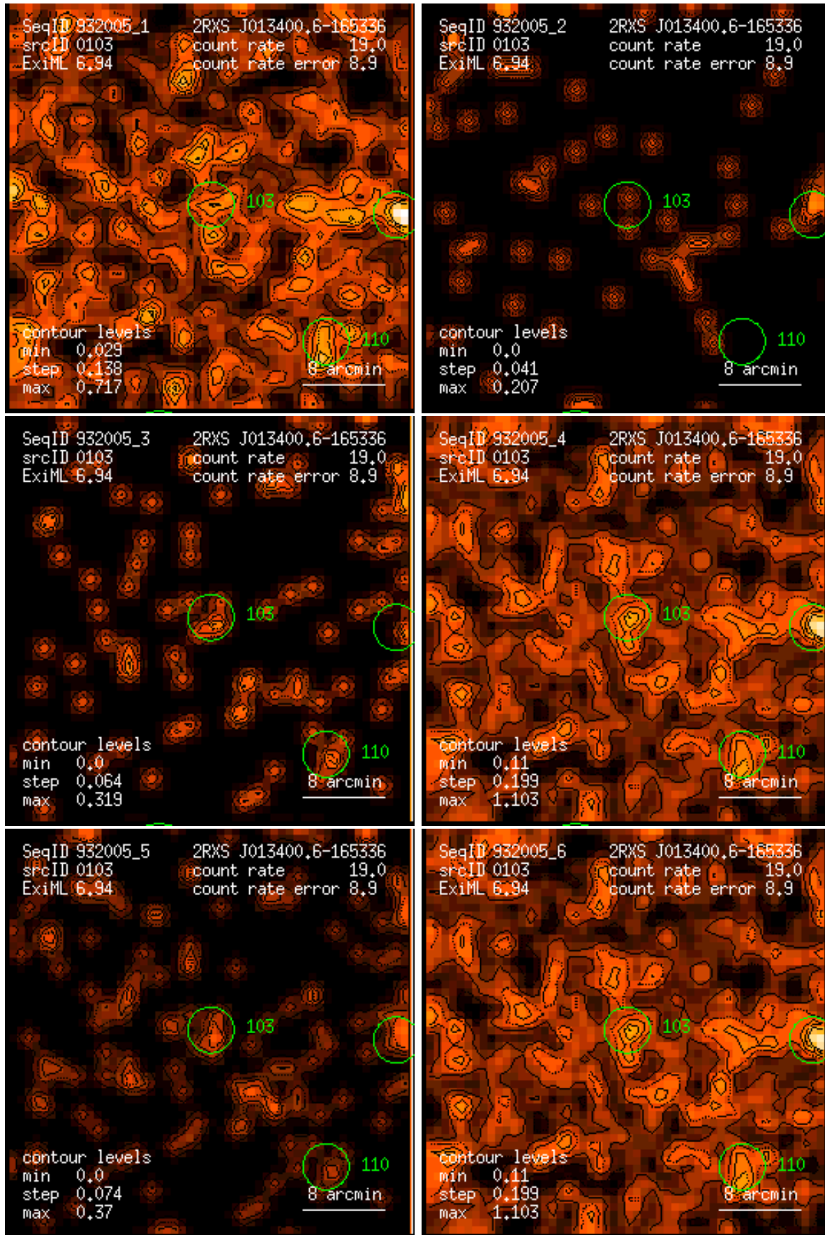
Figure 103: RASS 932005: detection 0103: band rate images, Gaussian filter: (1) PSPC channels 11 – 41, (2) 52 – 90, (3) 91 – 201, (4) 11 – 235, (5) 52 – 201, (6) 11 – 201. Broad band rates in counts/ks. Band rate contour levels in counts/ks/arcmin 2 .
