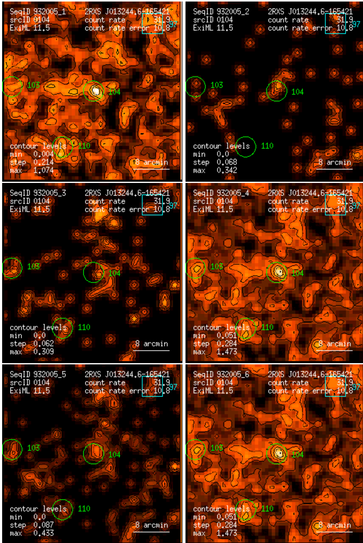
Figure 104: RASS 932005: detection 0104: band rate images, Gaussian filter: (1) PSPC channels 11 – 41, (2) 52 – 90, (3) 91 – 201, (4) 11 – 235, (5) 52 – 201, (6) 11 – 201. Broad band rates in counts/ks. Band rate contour levels in counts/ks/arcmin 2 .
