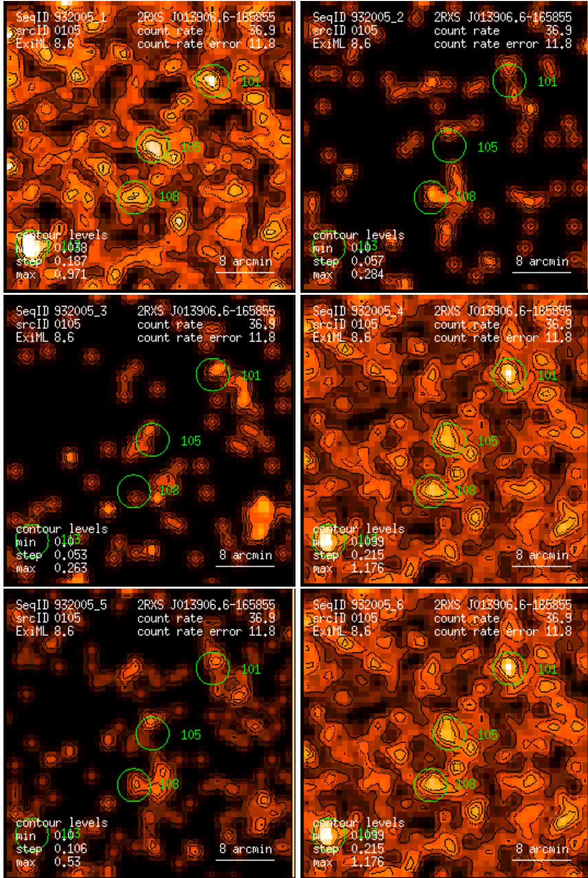
Figure 105: RASS 932005: detection 0105: band rate images, Gaussian filter: (1) PSPC channels 11 – 41, (2) 52 – 90, (3) 91 – 201, (4) 11 – 235, (5) 52 – 201, (6) 11 – 201. Broad band rates in counts/ks. Band rate contour levels in counts/ks/arcmin 2 .
