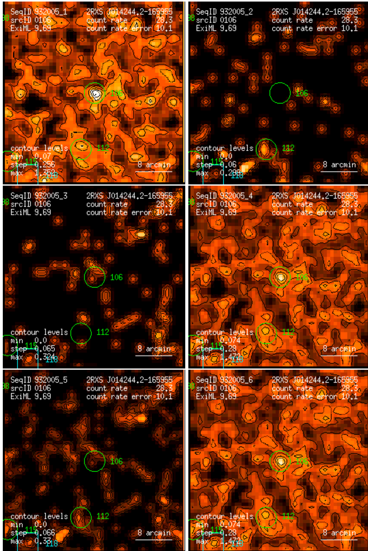
Figure 106: RASS 932005: detection 0106: band rate images, Gaussian filter: (1) PSPC channels 11 – 41, (2) 52 – 90, (3) 91 – 201, (4) 11 – 235, (5) 52 – 201, (6) 11 – 201. Broad band rates in counts/ks. Band rate contour levels in counts/ks/arcmin 2 .
