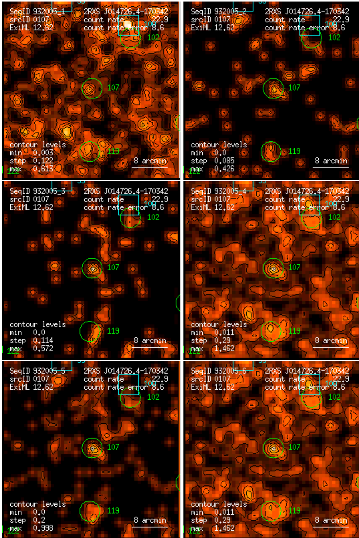
Figure 107: RASS 932005: detection 0107: band rate images, Gaussian filter: (1) PSPC channels 11 – 41, (2) 52 – 90, (3) 91 – 201, (4) 11 – 235, (5) 52 – 201, (6) 11 – 201. Broad band rates in counts/ks. Band rate contour levels in counts/ks/arcmin 2 .
