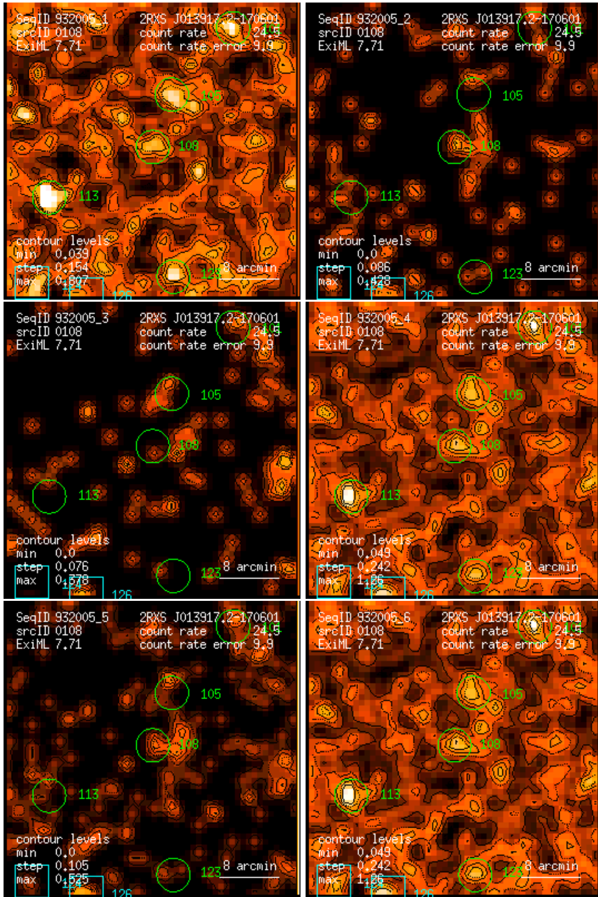
Figure 108: RASS 932005: detection 0108: band rate images, Gaussian filter: (1) PSPC channels 11 – 41, (2) 52 – 90, (3) 91 – 201, (4) 11 – 235, (5) 52 – 201, (6) 11 – 201. Broad band rates in counts/ks. Band rate contour levels in counts/ks/arcmin 2 .
