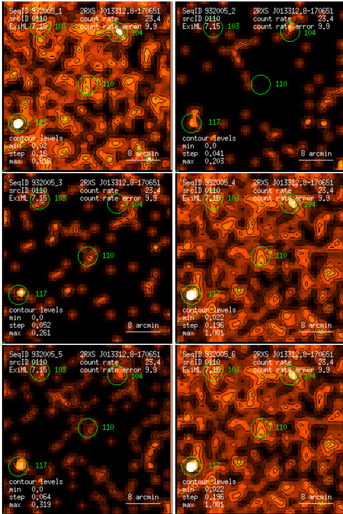
Figure 110: RASS 932005: detection 0110: band rate images, Gaussian filter: (1) PSPC channels 11 – 41, (2) 52 – 90, (3) 91 – 201, (4) 11 – 235, (5) 52 – 201, (6) 11 – 201. Broad band rates in counts/ks. Band rate contour levels in counts/ks/arcmin 2 .
