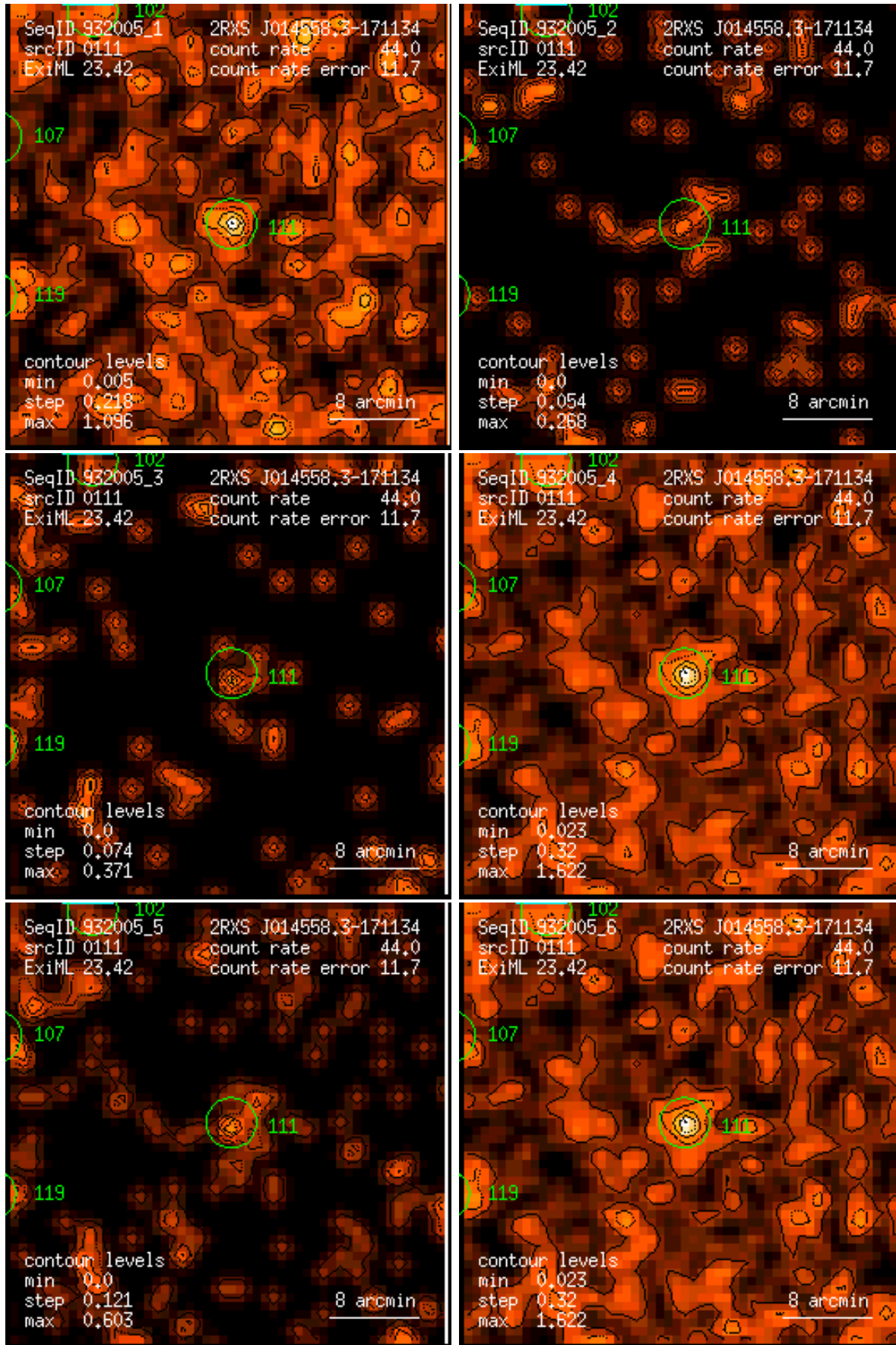
Figure 111: RASS 932005: detection 0111: band rate images, Gaussian filter: (1) PSPC channels 11 – 41, (2) 52 – 90, (3) 91 – 201, (4) 11 – 235, (5) 52 – 201, (6) 11 – 201. Broad band rates in counts/ks. Band rate contour levels in counts/ks/arcmin 2 .
