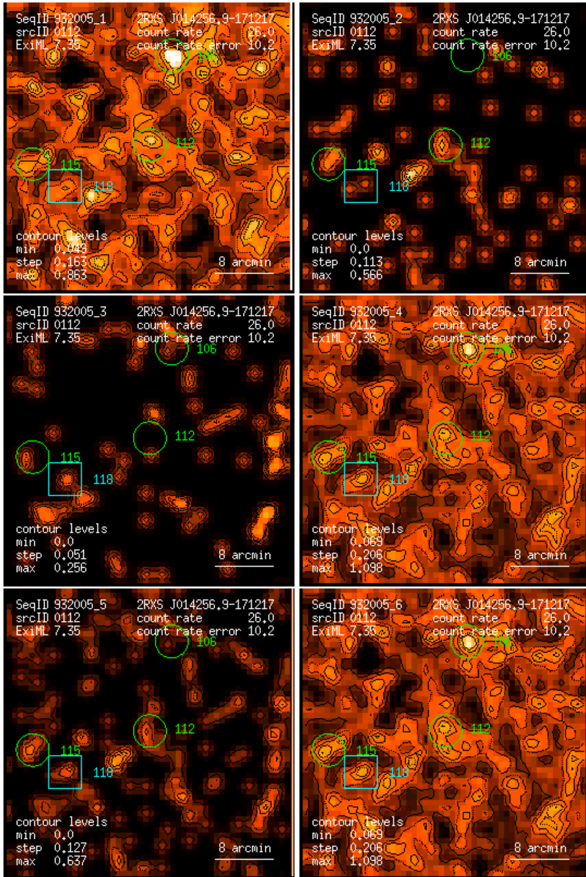
Figure 112: RASS 932005: detection 0112: band rate images, Gaussian filter: (1) PSPC channels 11 – 41, (2) 52 – 90, (3) 91 – 201, (4) 11 – 235, (5) 52 – 201, (6) 11 – 201. Broad band rates in counts/ks. Band rate contour levels in counts/ks/arcmin 2 .
