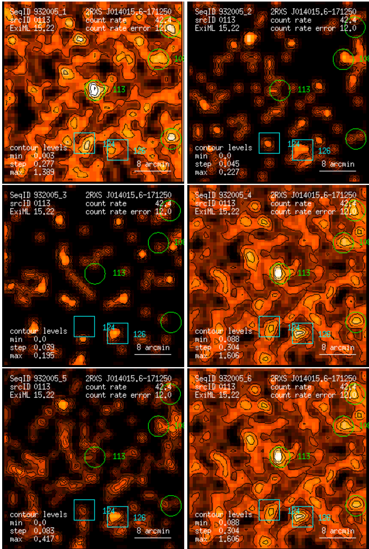
Figure 113: RASS 932005: detection 0113: band rate images, Gaussian filter: (1) PSPC channels 11 – 41, (2) 52 – 90, (3) 91 – 201, (4) 11 – 235, (5) 52 – 201, (6) 11 – 201. Broad band rates in counts/ks. Band rate contour levels in counts/ks/arcmin 2 .
