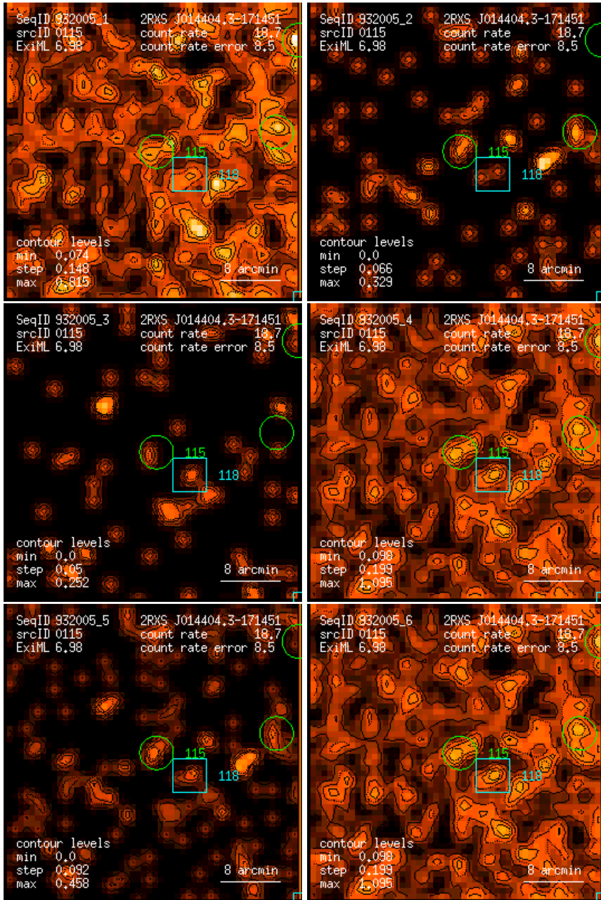
Figure 115: RASS 932005: detection 0115: band rate images, Gaussian filter: (1) PSPC channels 11 – 41, (2) 52 – 90, (3) 91 – 201, (4) 11 – 235, (5) 52 – 201, (6) 11 – 201. Broad band rates in counts/ks. Band rate contour levels in counts/ks/arcmin 2 .
