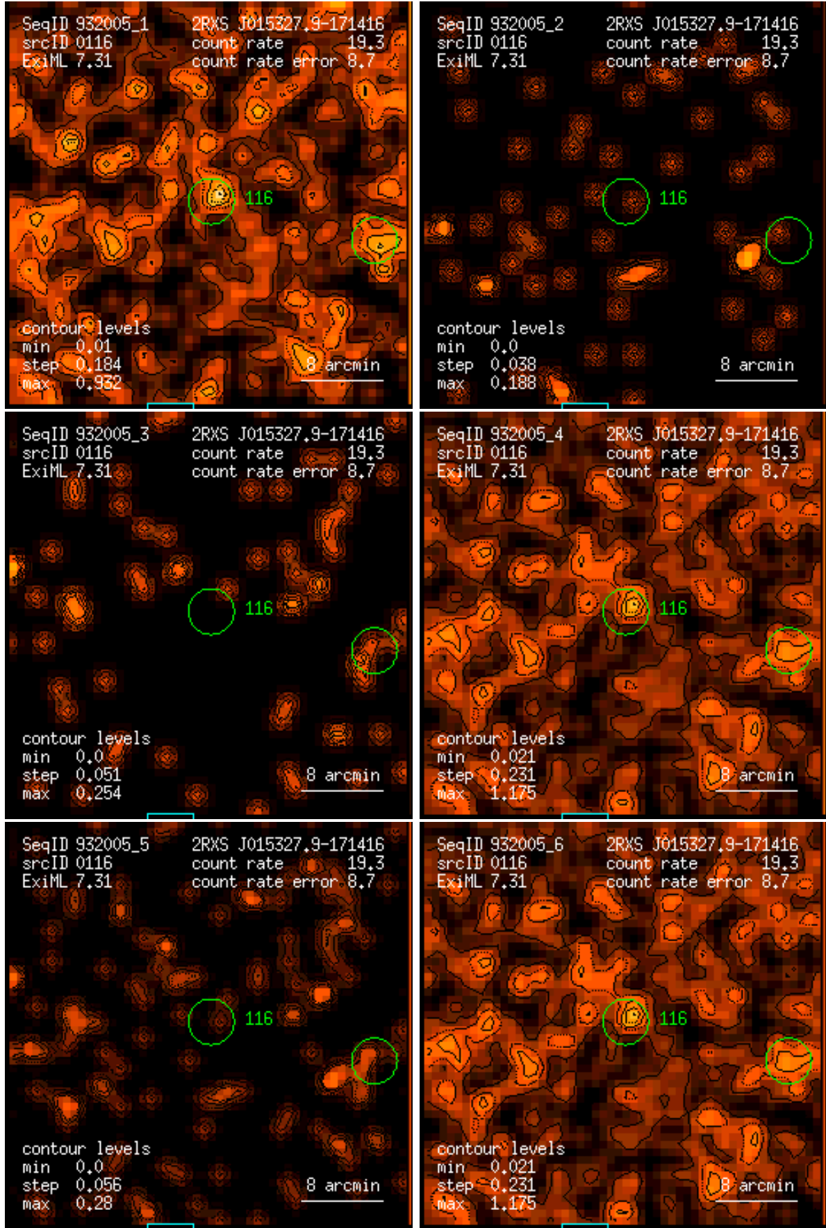
Figure 116: RASS 932005: detection 0116: band rate images, Gaussian filter: (1) PSPC channels 11 – 41, (2) 52 – 90, (3) 91 – 201, (4) 11 – 235, (5) 52 – 201, (6) 11 – 201. Broad band rates in counts/ks. Band rate contour levels in counts/ks/arcmin 2 .
