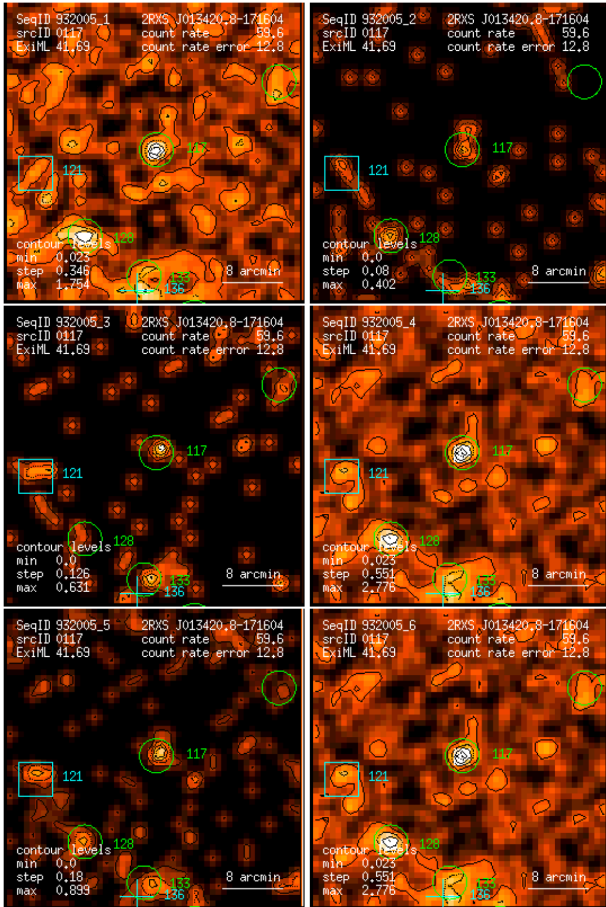
Figure 117: RASS 932005: detection 0117: band rate images, Gaussian filter: (1) PSPC channels 11 – 41, (2) 52 – 90, (3) 91 – 201, (4) 11 – 235, (5) 52 – 201, (6) 11 – 201. Broad band rates in counts/ks. Band rate contour levels in counts/ks/arcmin 2 .
