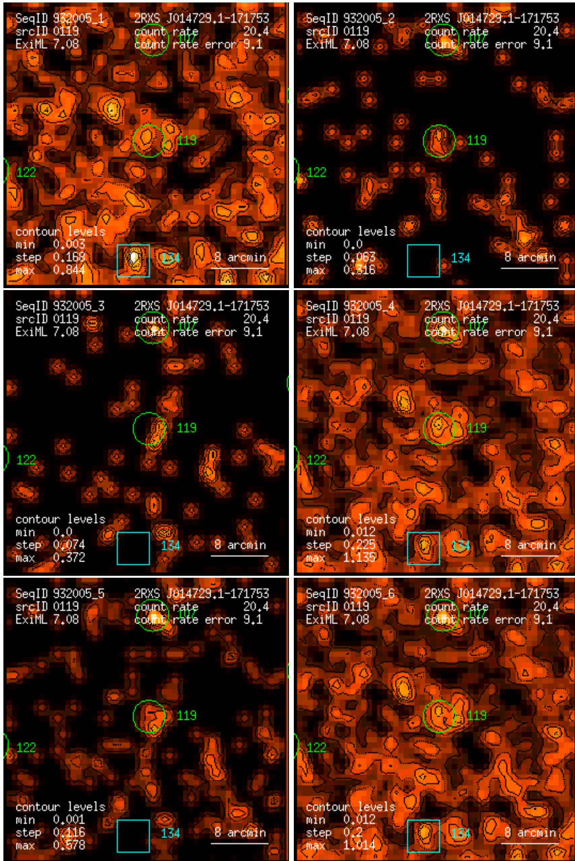
Figure 119: RASS 932005: detection 0119: band rate images, Gaussian filter: (1) PSPC channels 11 – 41, (2) 52 – 90, (3) 91 – 201, (4) 11 – 235, (5) 52 – 201, (6) 11 – 201. Broad band rates in counts/ks. Band rate contour levels in counts/ks/arcmin 2 .
