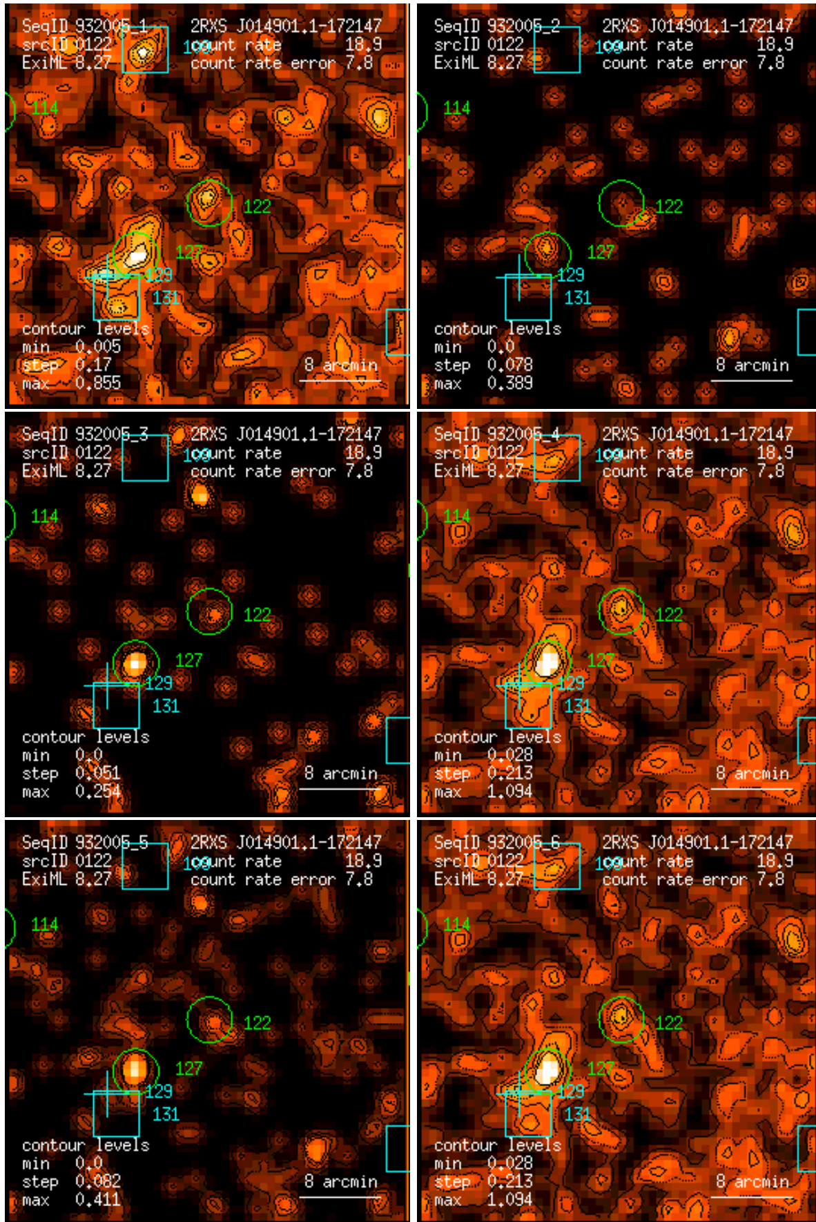
Figure 122: RASS 932005: detection 0122: band rate images, Gaussian filter: (1) PSPC channels 11 – 41, (2) 52 – 90, (3) 91 – 201, (4) 11 – 235, (5) 52 – 201, (6) 11 – 201. Broad band rates in counts/ks. Band rate contour levels in counts/ks/arcmin 2 .
