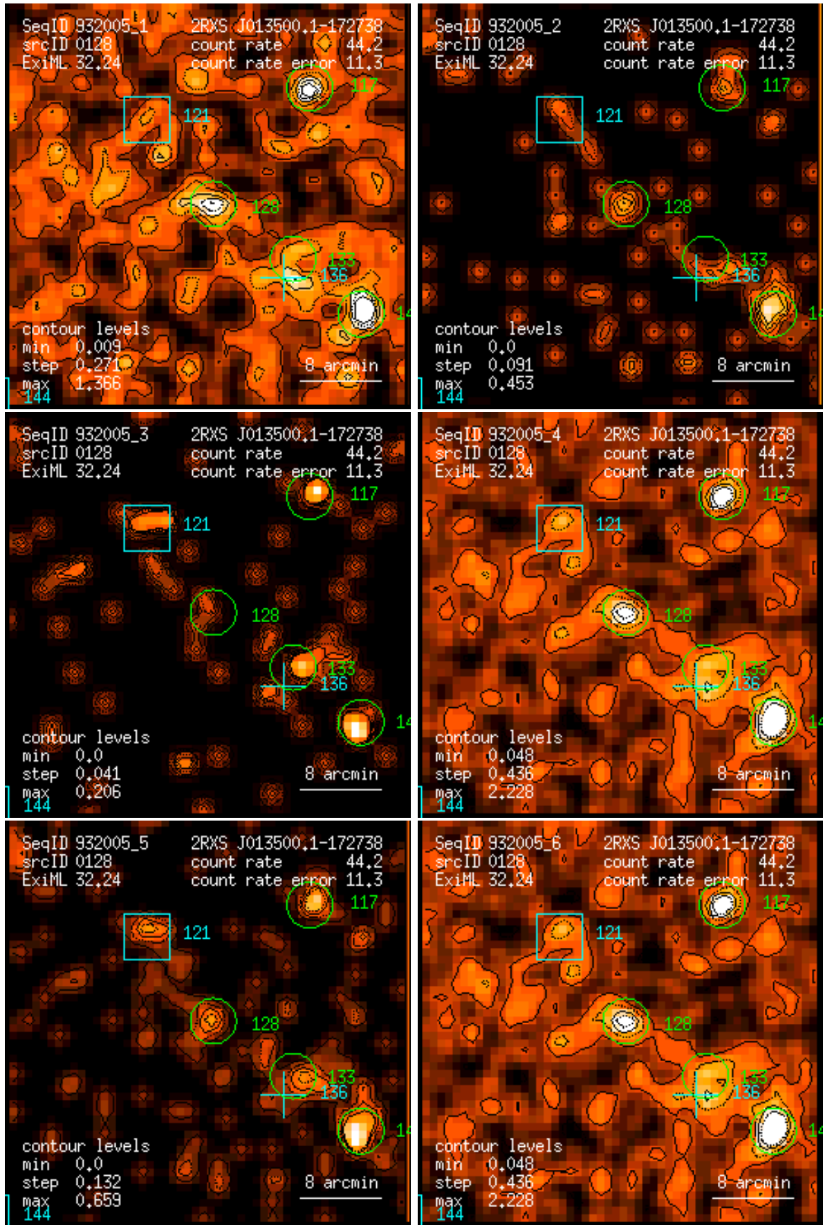
Figure 128: RASS 932005: detection 0128: band rate images, Gaussian filter: (1) PSPC channels 11 – 41, (2) 52 – 90, (3) 91 – 201, (4) 11 – 235, (5) 52 – 201, (6) 11 – 201. Broad band rates in counts/ks. Band rate contour levels in counts/ks/arcmin 2 .
