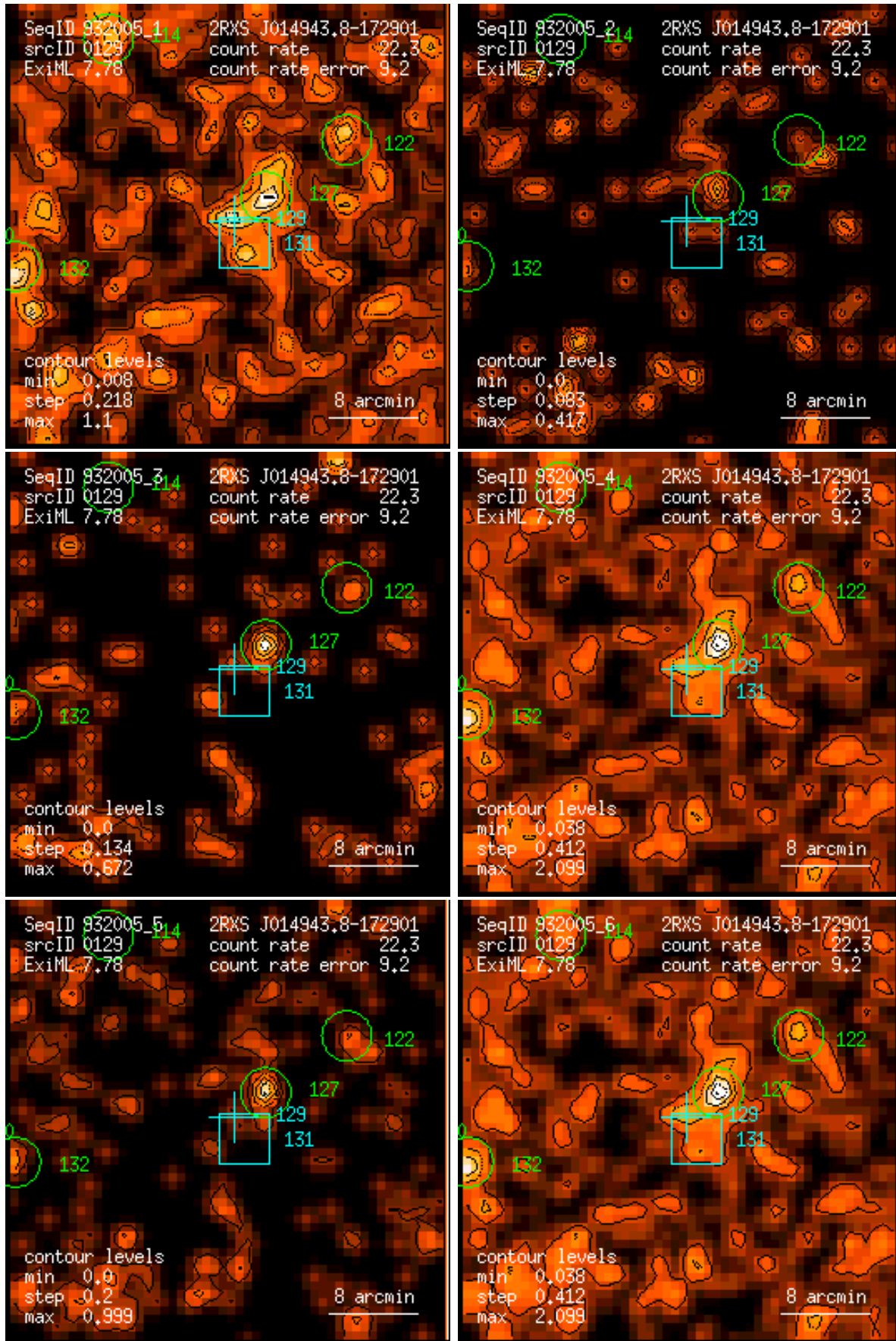
Figure 129: RASS 932005: detection 0129: band rate images, Gaussian filter: (1) PSPC channels 11 – 41, (2) 52 – 90, (3) 91 – 201, (4) 11 – 235, (5) 52 – 201, (6) 11 – 201. Broad band rates in counts/ks. Band rate contour levels in counts/ks/arcmin 2 .
