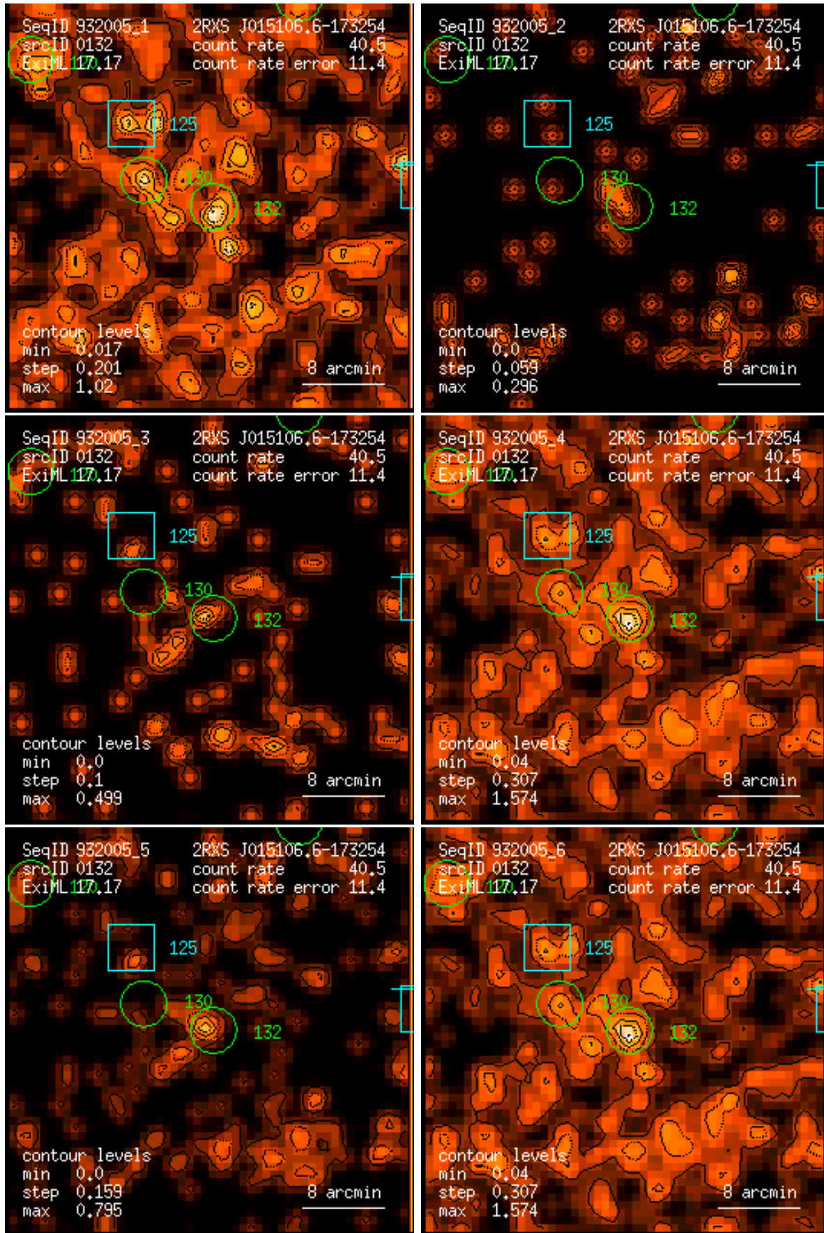
Figure 132: RASS 932005: detection 0132: band rate images, Gaussian filter: (1) PSPC channels 11 – 41, (2) 52 – 90, (3) 91 – 201, (4) 11 – 235, (5) 52 – 201, (6) 11 – 201. Broad band rates in counts/ks. Band rate contour levels in counts/ks/arcmin 2 .
