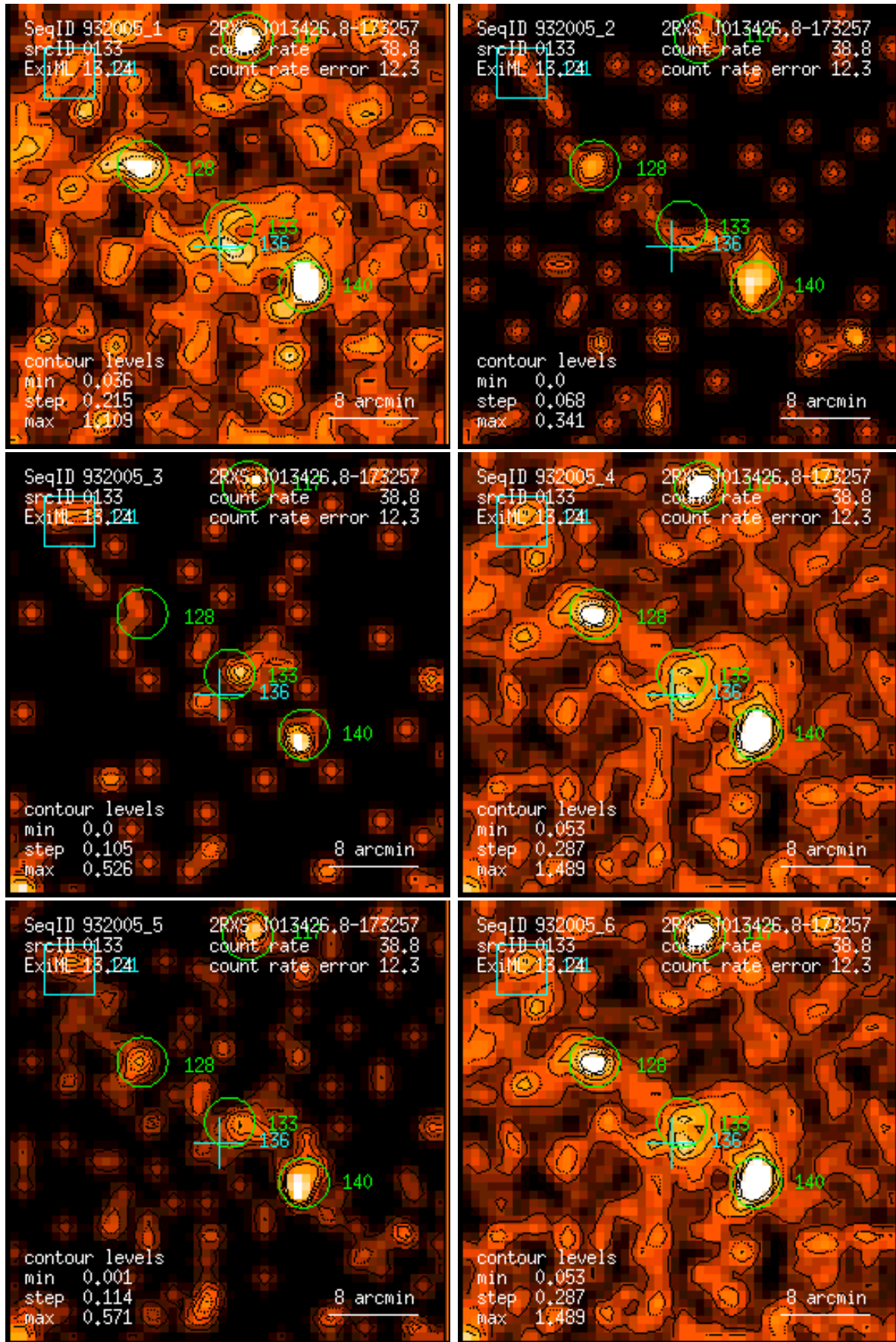
Figure 133: RASS 932005: detection 0133: band rate images, Gaussian filter: (1) PSPC channels 11 – 41, (2) 52 – 90, (3) 91 – 201, (4) 11 – 235, (5) 52 – 201, (6) 11 – 201. Broad band rates in counts/ks. Band rate contour levels in counts/ks/arcmin 2 .
