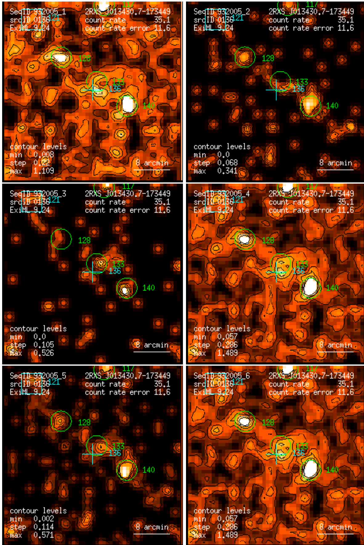
Figure 136: RASS 932005: detection 0136: band rate images, Gaussian filter: (1) PSPC channels 11 – 41, (2) 52 – 90, (3) 91 – 201, (4) 11 – 235, (5) 52 – 201, (6) 11 – 201. Broad band rates in counts/ks. Band rate contour levels in counts/ks/arcmin 2 .
