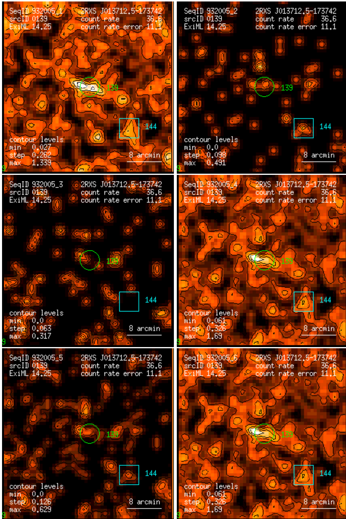
Figure 139: RASS 932005: detection 0139: band rate images, Gaussian filter: (1) PSPC channels 11 – 41, (2) 52 – 90, (3) 91 – 201, (4) 11 – 235, (5) 52 – 201, (6) 11 – 201. Broad band rates in counts/ks. Band rate contour levels in counts/ks/arcmin 2 .
