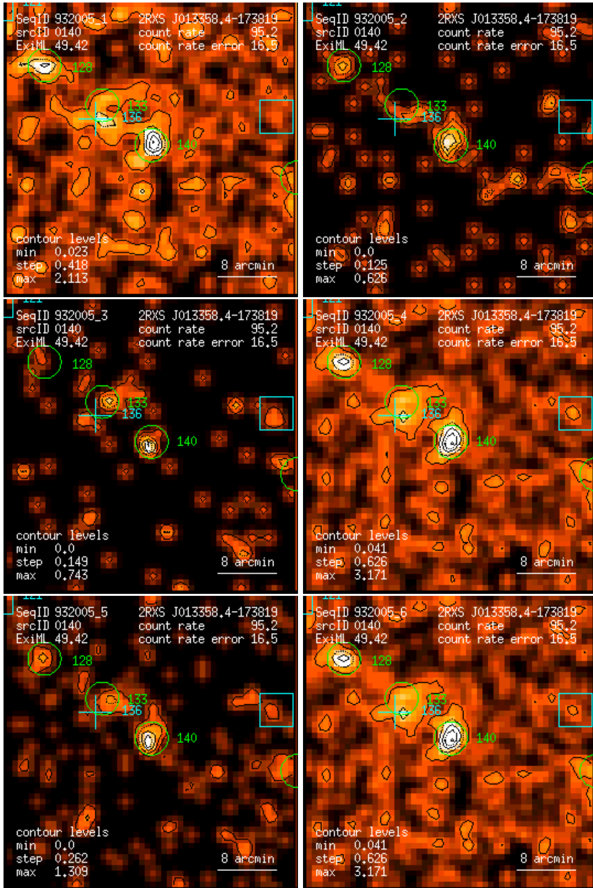
Figure 140: RASS 932005: detection 0140: band rate images, Gaussian filter: (1) PSPC channels 11 – 41, (2) 52 – 90, (3) 91 – 201, (4) 11 – 235, (5) 52 – 201, (6) 11 – 201. Broad band rates in counts/ks. Band rate contour levels in counts/ks/arcmin 2 .
