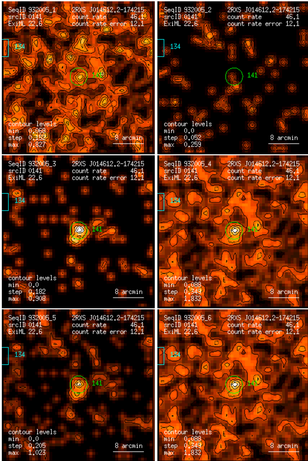
Figure 141: RASS 932005: detection 0141: band rate images, Gaussian filter: (1) PSPC channels 11 – 41, (2) 52 – 90, (3) 91 – 201, (4) 11 – 235, (5) 52 – 201, (6) 11 – 201. Broad band rates in counts/ks. Band rate contour levels in counts/ks/arcmin 2 .
