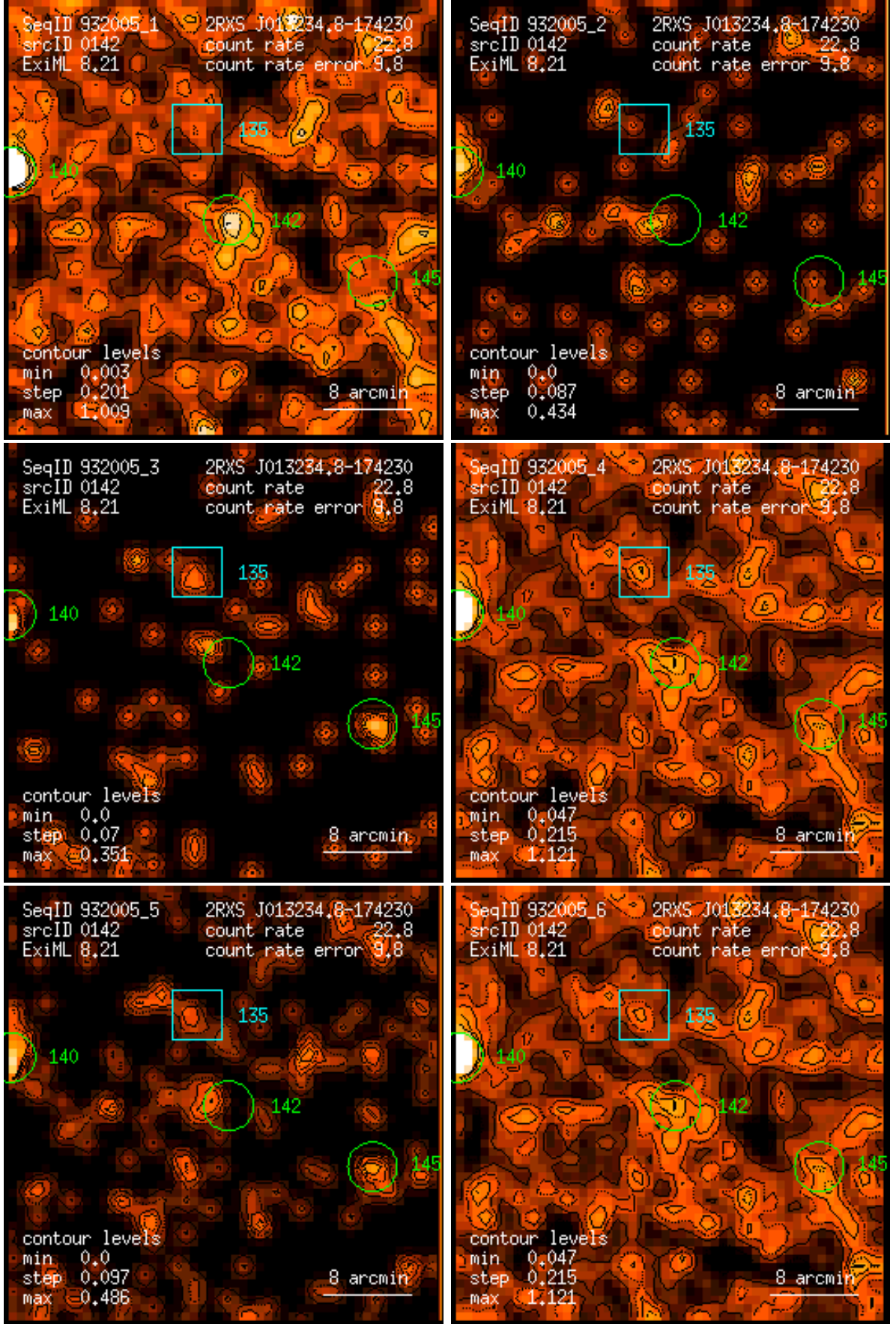
Figure 142: RASS 932005: detection 0142: band rate images, Gaussian filter: (1) PSPC channels 11 – 41, (2) 52 – 90, (3) 91 – 201, (4) 11 – 235, (5) 52 – 201, (6) 11 – 201. Broad band rates in counts/ks. Band rate contour levels in counts/ks/arcmin 2 .
