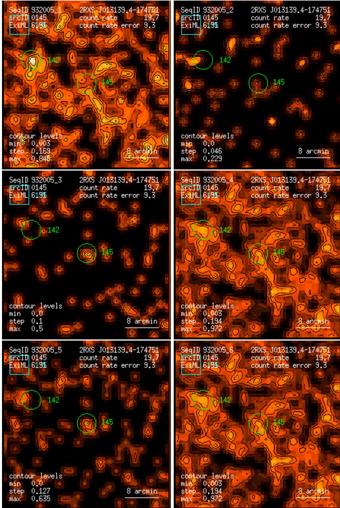
Figure 145: RASS 932005: detection 0145: band rate images, Gaussian filter: (1) PSPC channels 11 – 41, (2) 52 – 90, (3) 91 – 201, (4) 11 – 235, (5) 52 – 201, (6) 11 – 201. Broad band rates in counts/ks. Band rate contour levels in counts/ks/arcmin 2 .
