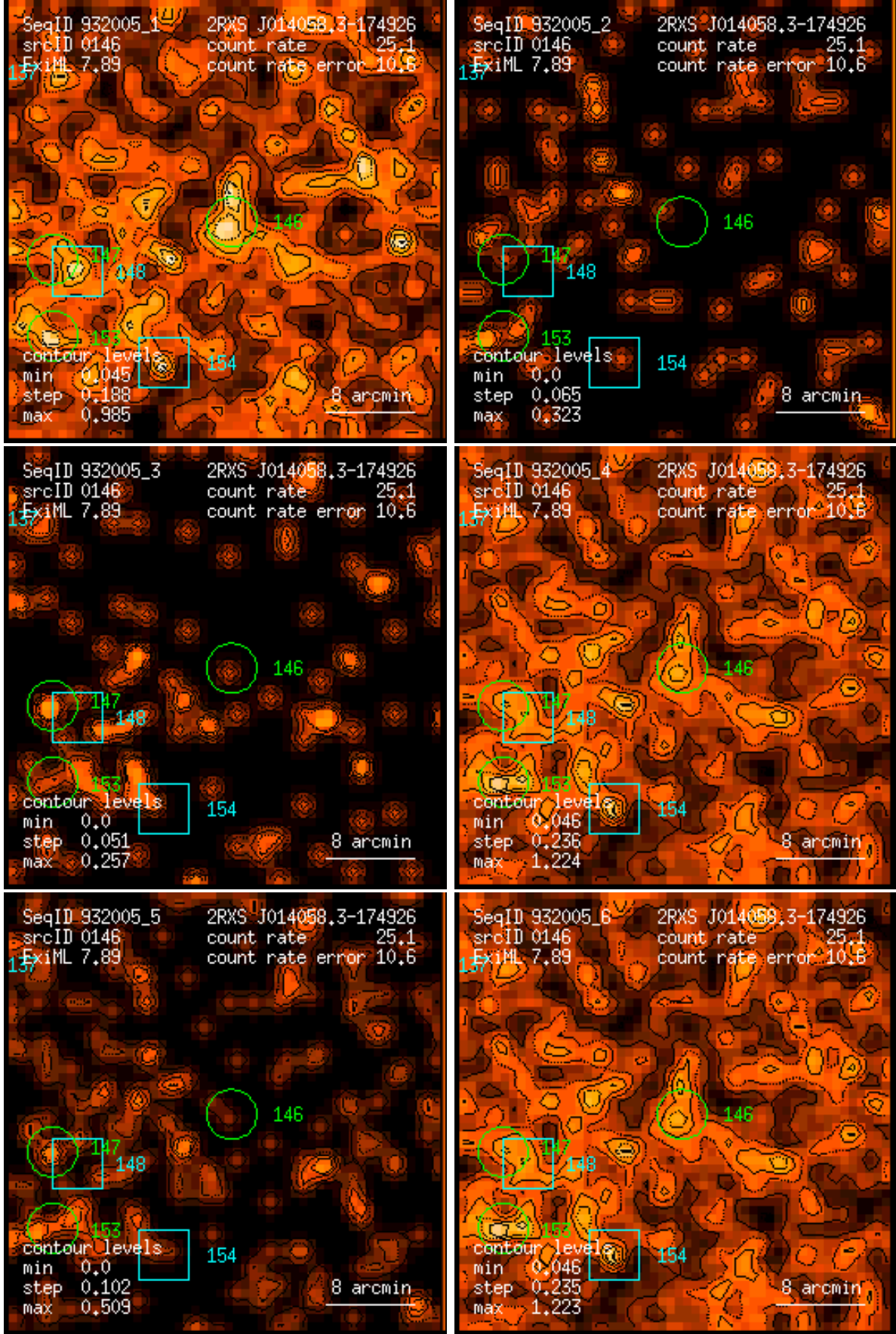
Figure 146: RASS 932005: detection 0146: band rate images, Gaussian filter: (1) PSPC channels 11 – 41, (2) 52 – 90, (3) 91 – 201, (4) 11 – 235, (5) 52 – 201, (6) 11 – 201. Broad band rates in counts/ks. Band rate contour levels in counts/ks/arcmin 2 .
