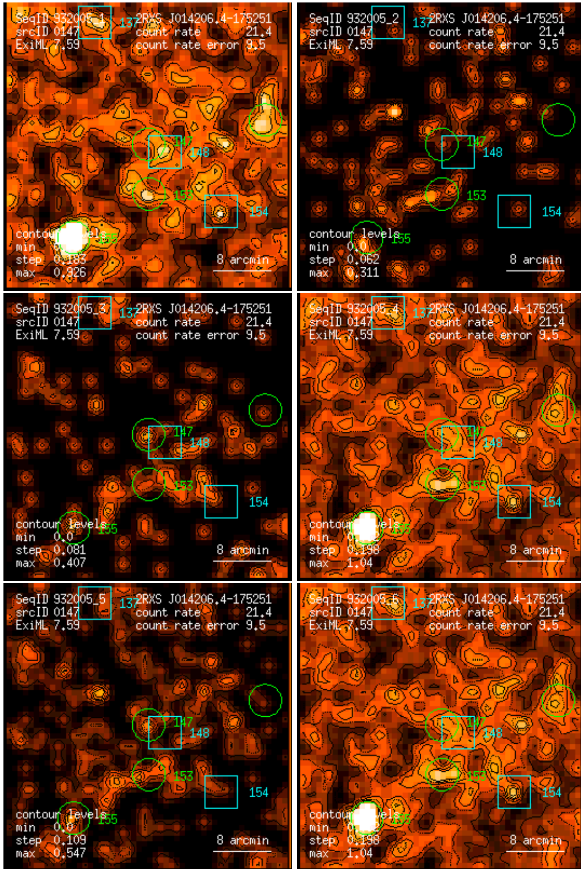
Figure 147: RASS 932005: detection 0147: band rate images, Gaussian filter: (1) PSPC channels 11 – 41, (2) 52 – 90, (3) 91 – 201, (4) 11 – 235, (5) 52 – 201, (6) 11 – 201. Broad band rates in counts/ks. Band rate contour levels in counts/ks/arcmin 2 .
