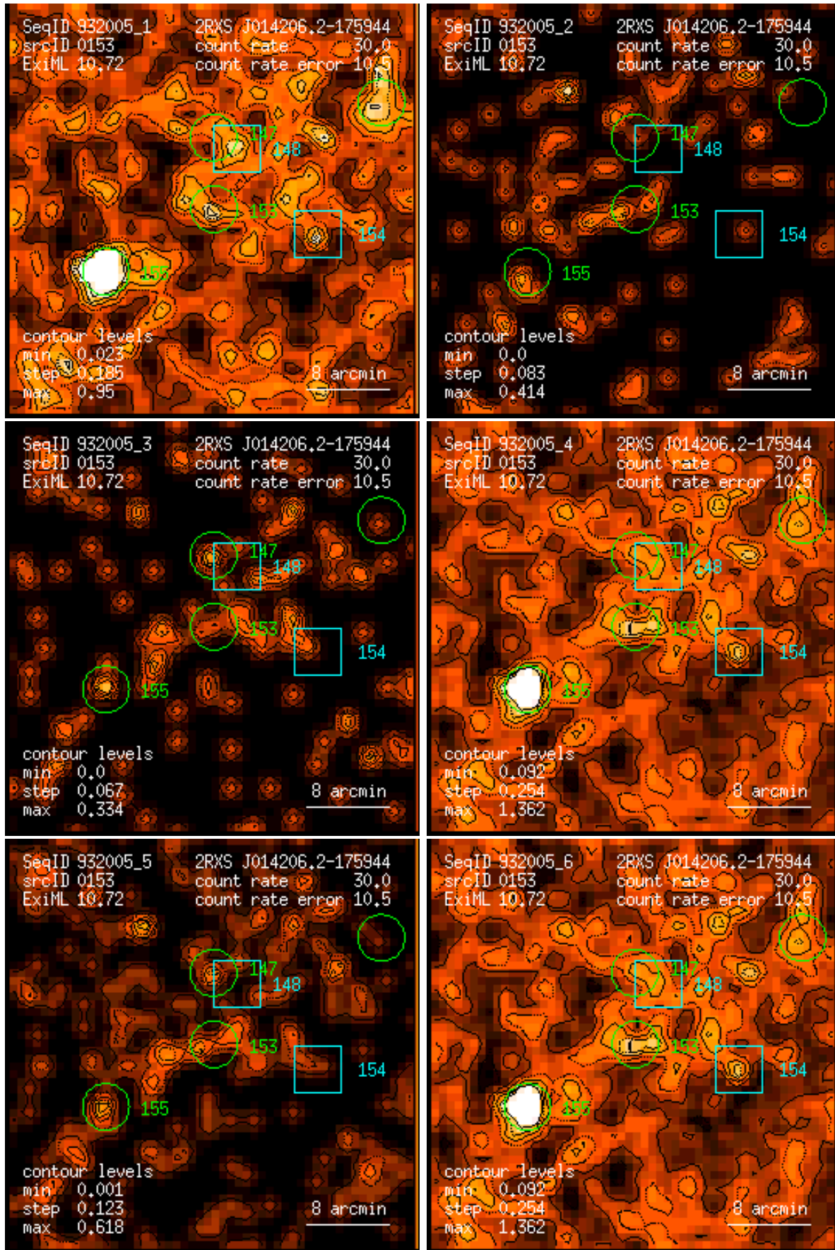
Figure 153: RASS 932005: detection 0153: band rate images, Gaussian filter: (1) PSPC channels 11 – 41, (2) 52 – 90, (3) 91 – 201, (4) 11 – 235, (5) 52 – 201, (6) 11 – 201. Broad band rates in counts/ks. Band rate contour levels in counts/ks/arcmin 2 .
