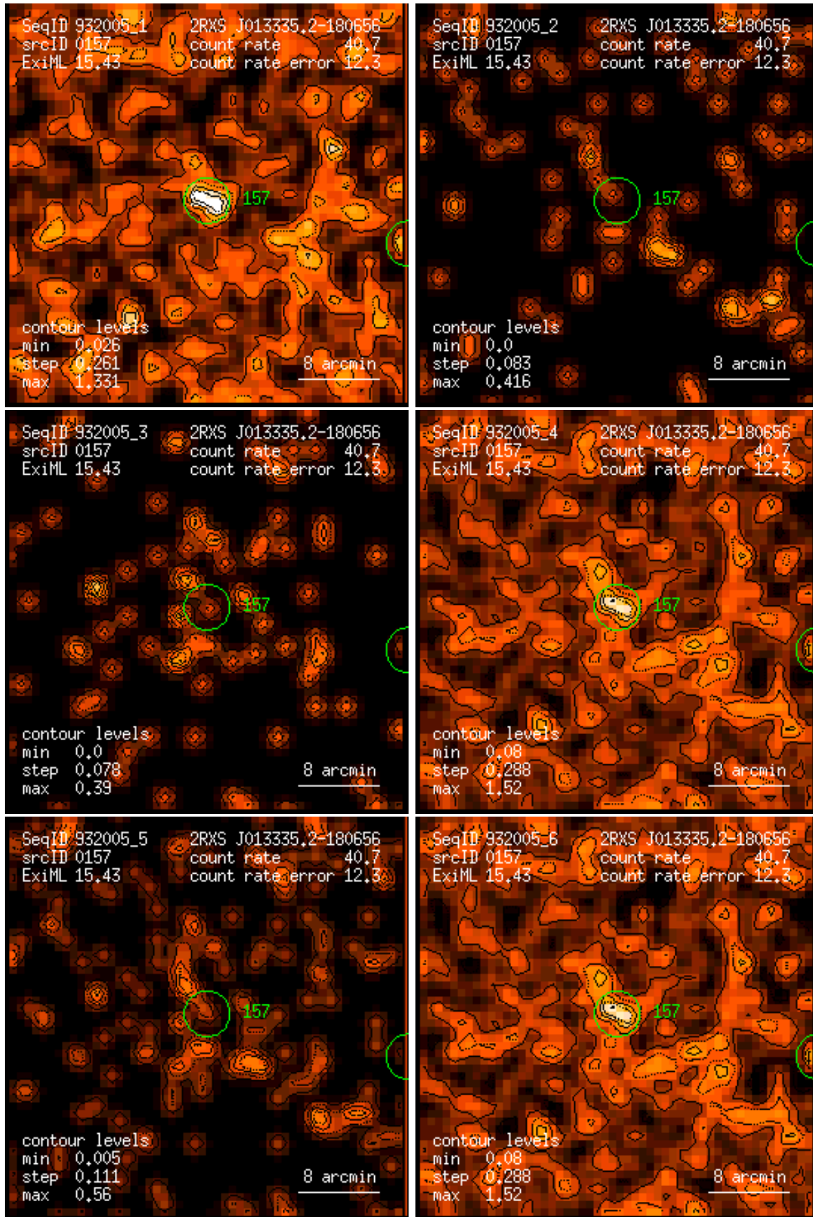
Figure 157: RASS 932005: detection 0157: band rate images, Gaussian filter: (1) PSPC channels 11 – 41, (2) 52 – 90, (3) 91 – 201, (4) 11 – 235, (5) 52 – 201, (6) 11 – 201. Broad band rates in counts/ks. Band rate contour levels in counts/ks/arcmin 2 .
