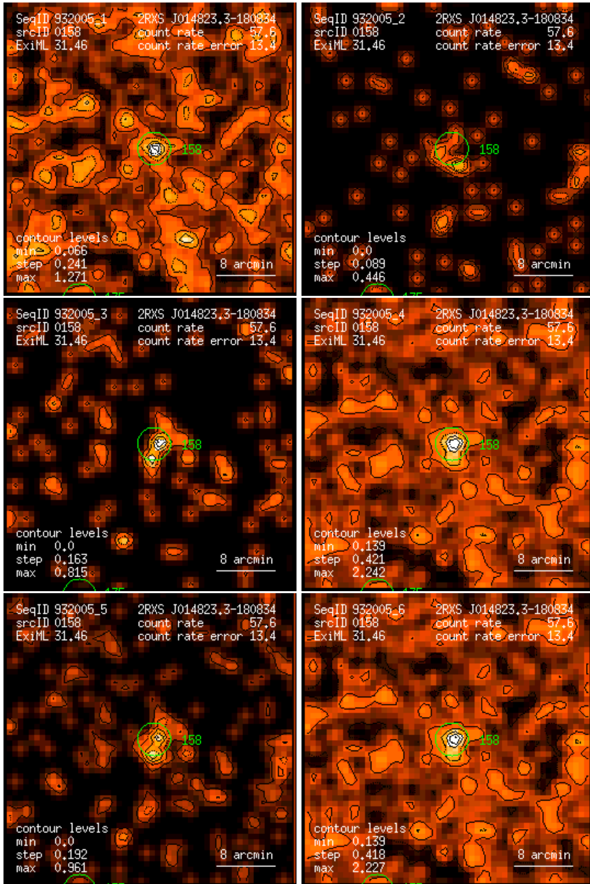
Figure 158: RASS 932005: detection 0158: band rate images, Gaussian filter: (1) PSPC channels 11 – 41, (2) 52 – 90, (3) 91 – 201, (4) 11 – 235, (5) 52 – 201, (6) 11 – 201. Broad band rates in counts/ks. Band rate contour levels in counts/ks/arcmin 2 .
