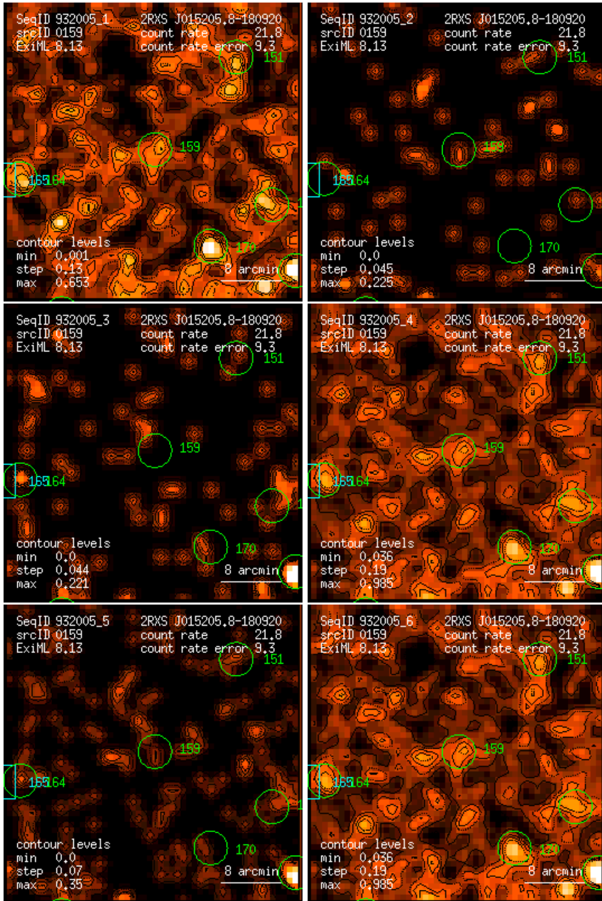
Figure 159: RASS 932005: detection 0159: band rate images, Gaussian filter: (1) PSPC channels 11 – 41, (2) 52 – 90, (3) 91 – 201, (4) 11 – 235, (5) 52 – 201, (6) 11 – 201. Broad band rates in counts/ks. Band rate contour levels in counts/ks/arcmin 2 .
